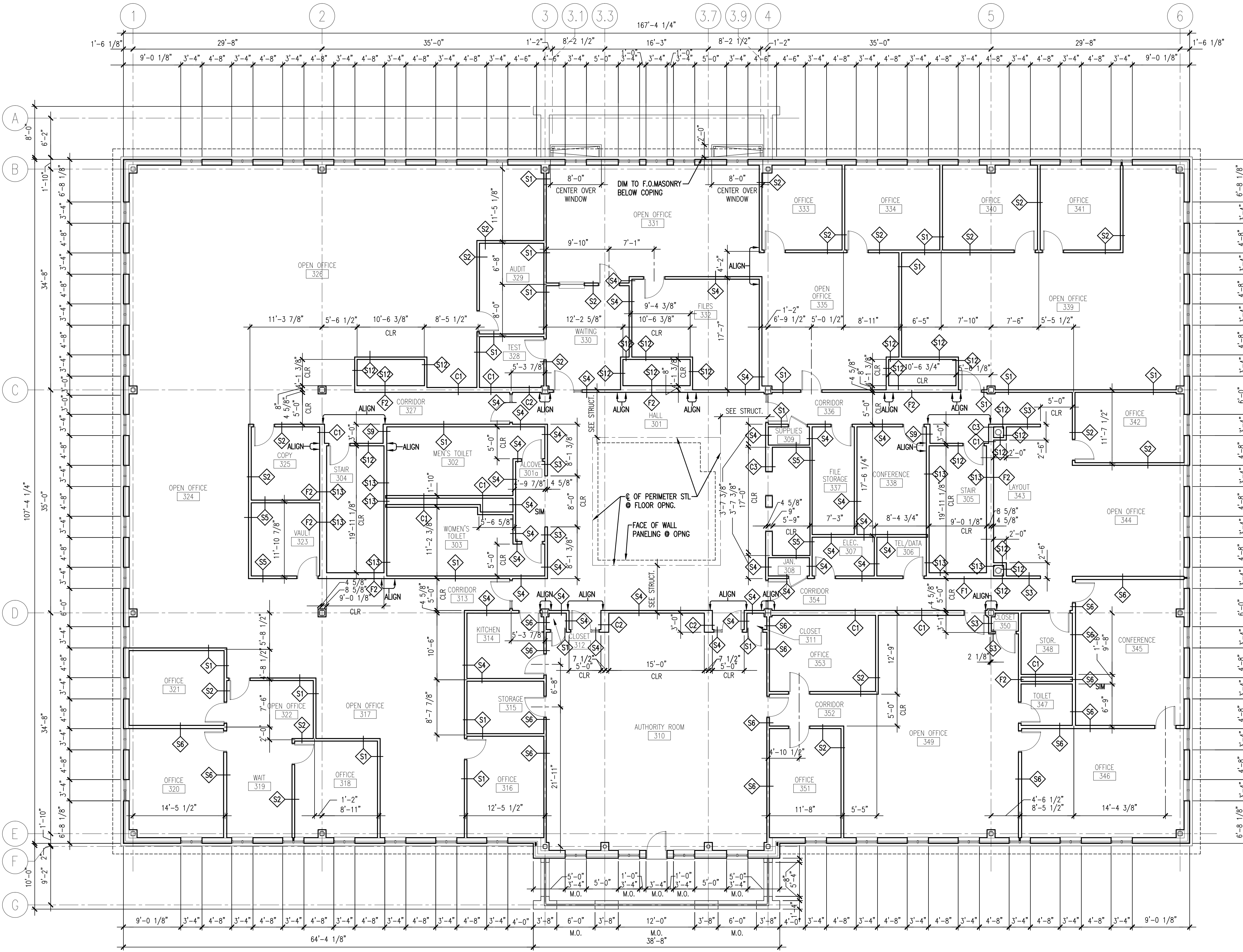
A1 THIRD FLOOR LAYOUT PLAN
