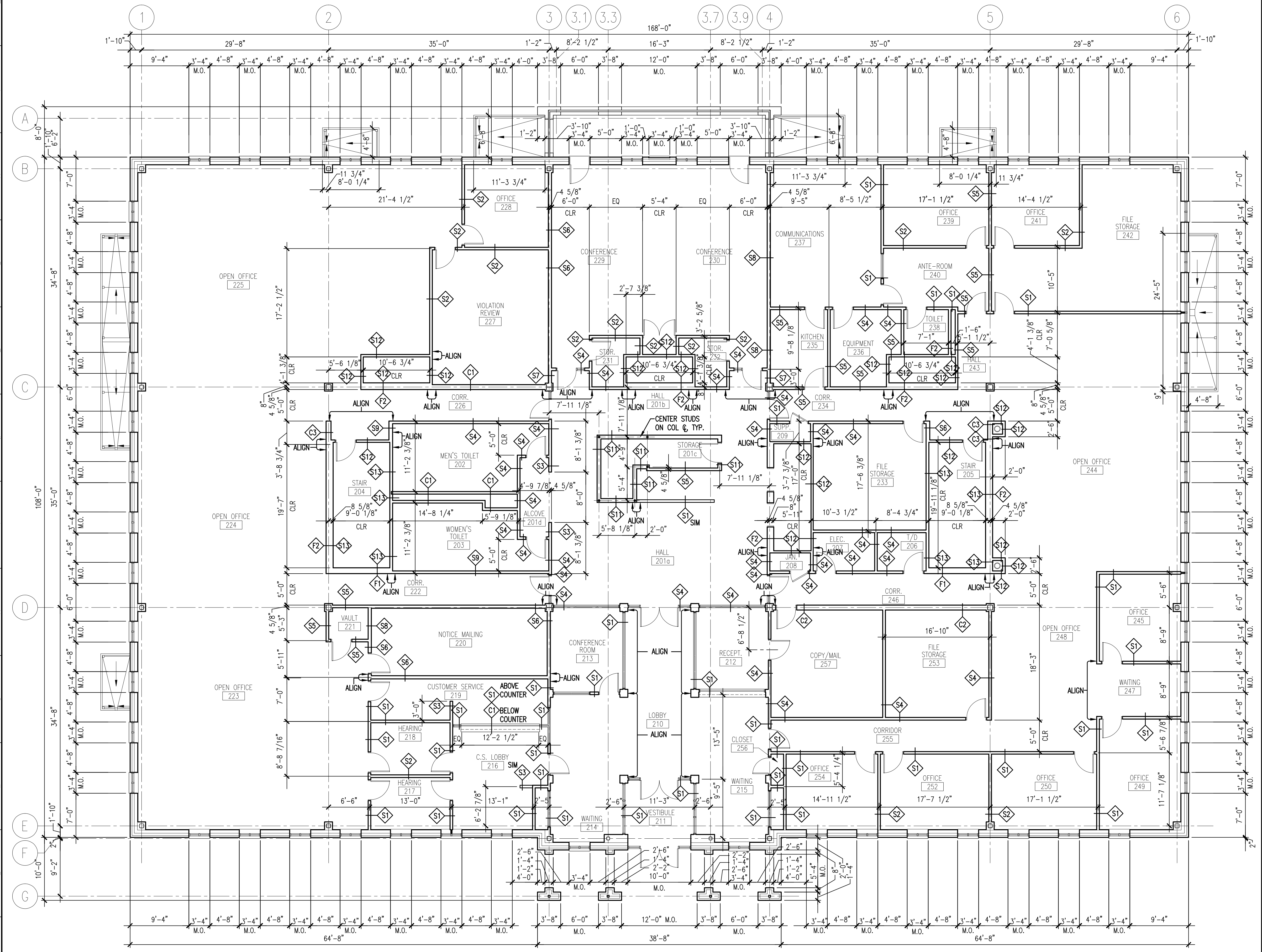
A1 SECOND FLOOR LAYOUT PLAN
