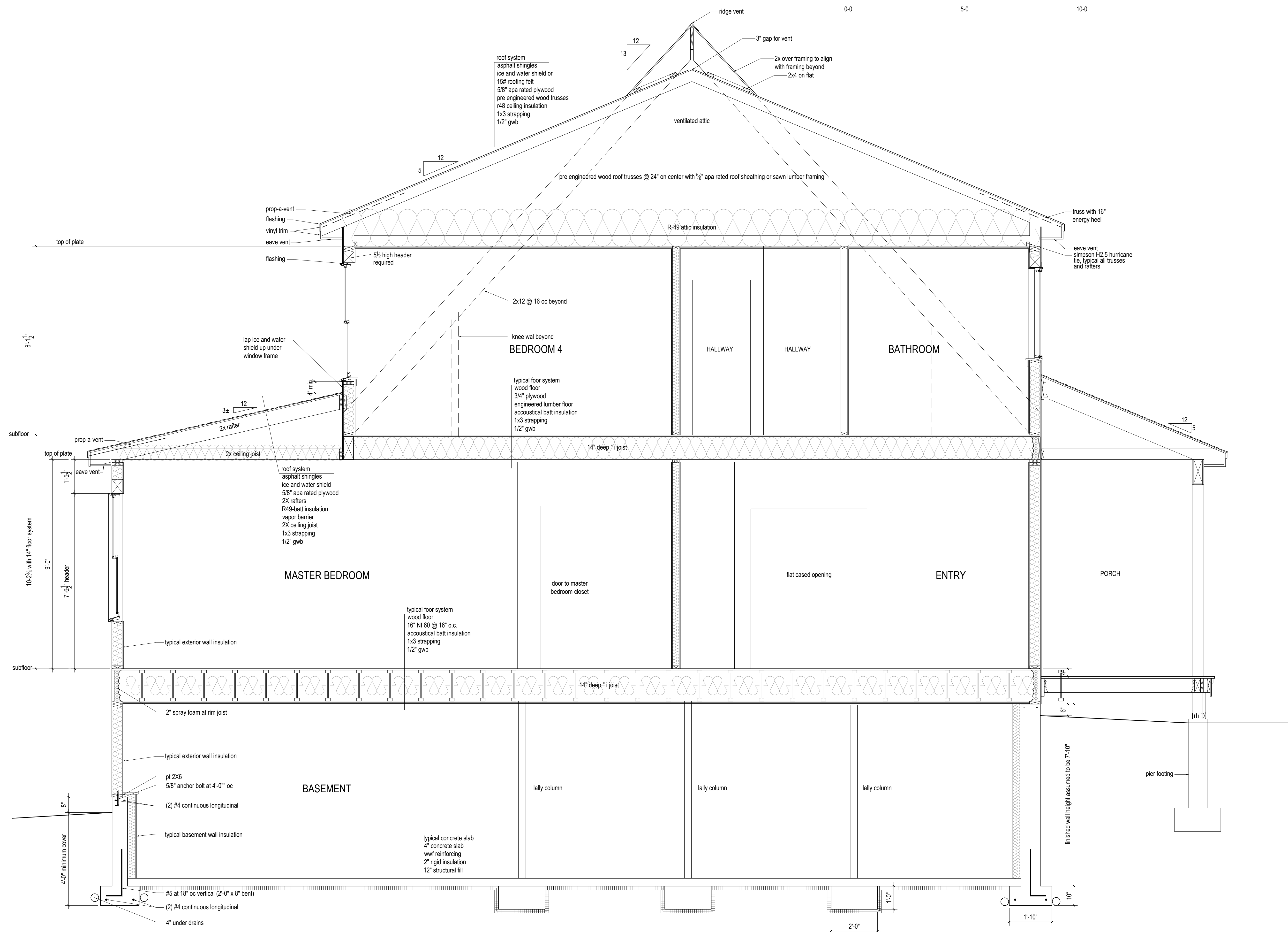
1 Building Section scale: 1/2" = 1'-0"
