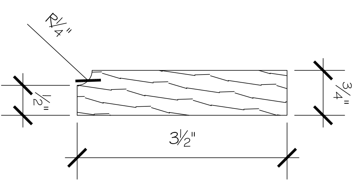
APRON 1X4 POPLAR WITH ROUTED EDGE 3/4" X 3 1/2"
