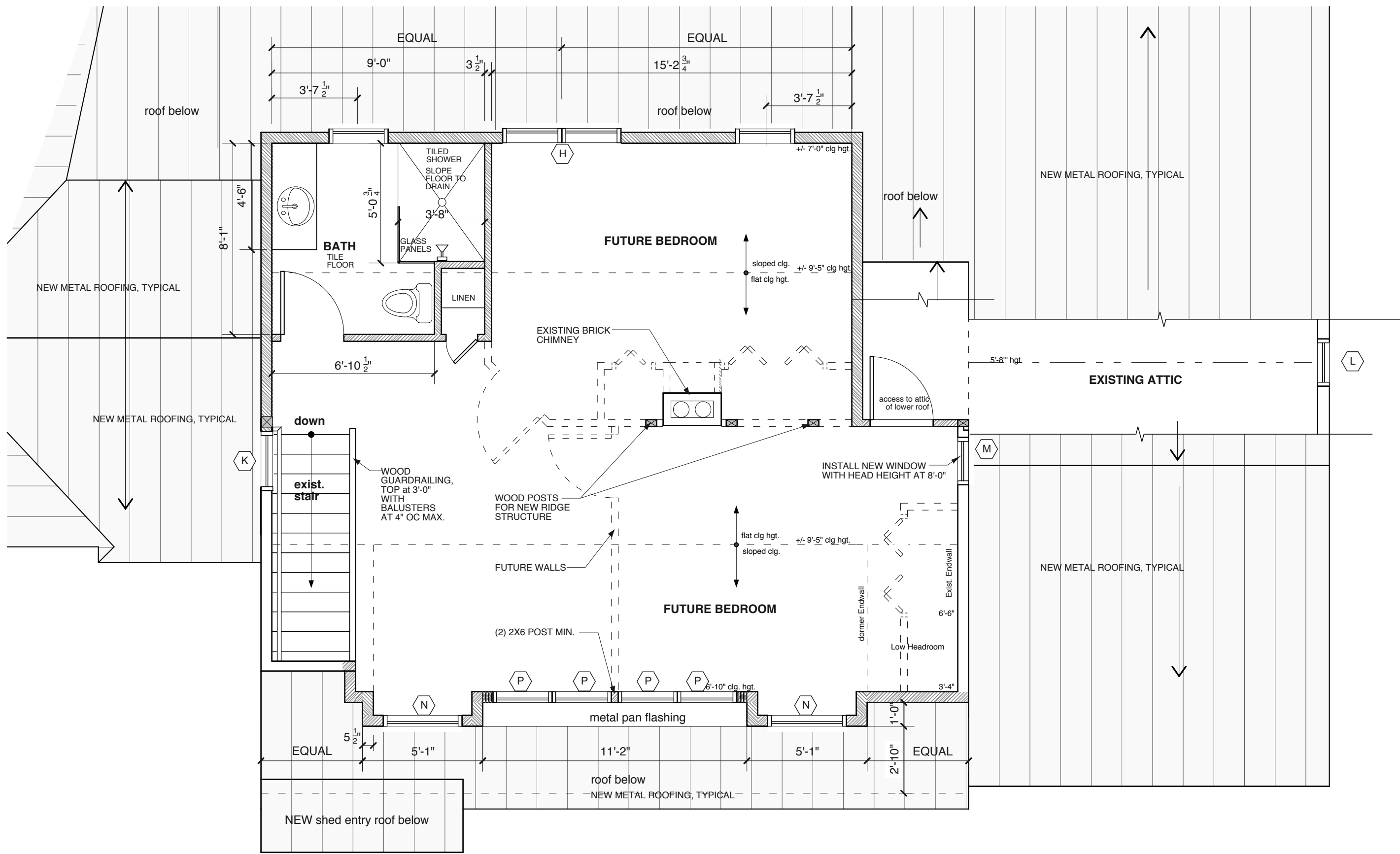
SECOND FLOOR PROPOSED PLAN SCALE: 1/4" = 1'-0" ref: sheet A1.2 4 0 2 4 8 Scale: 1/4 inch = 1 foot
