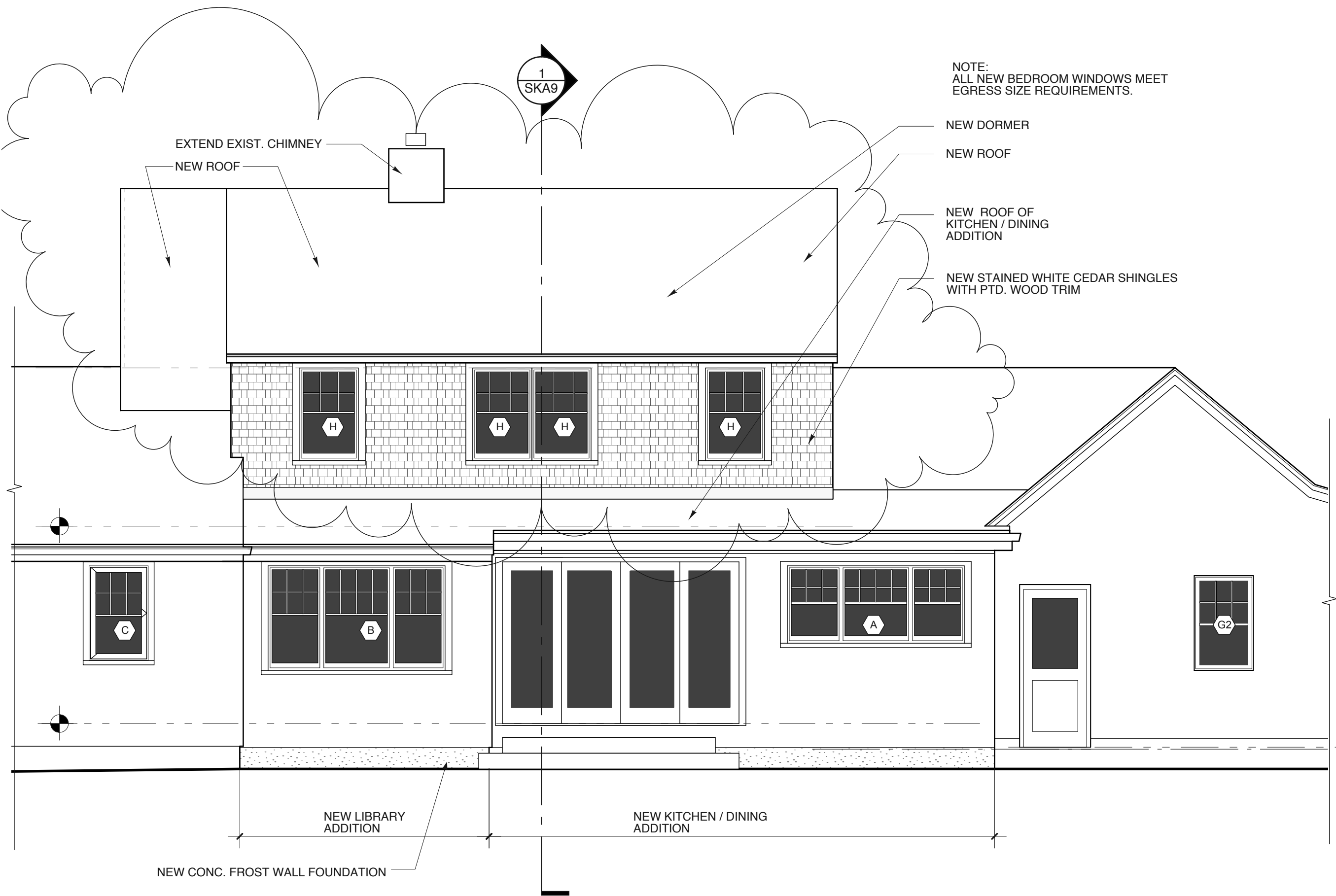
WEST ELEVATION (rear) SCALE: 1/4" = 1'-0" ref: sheet A2.2
