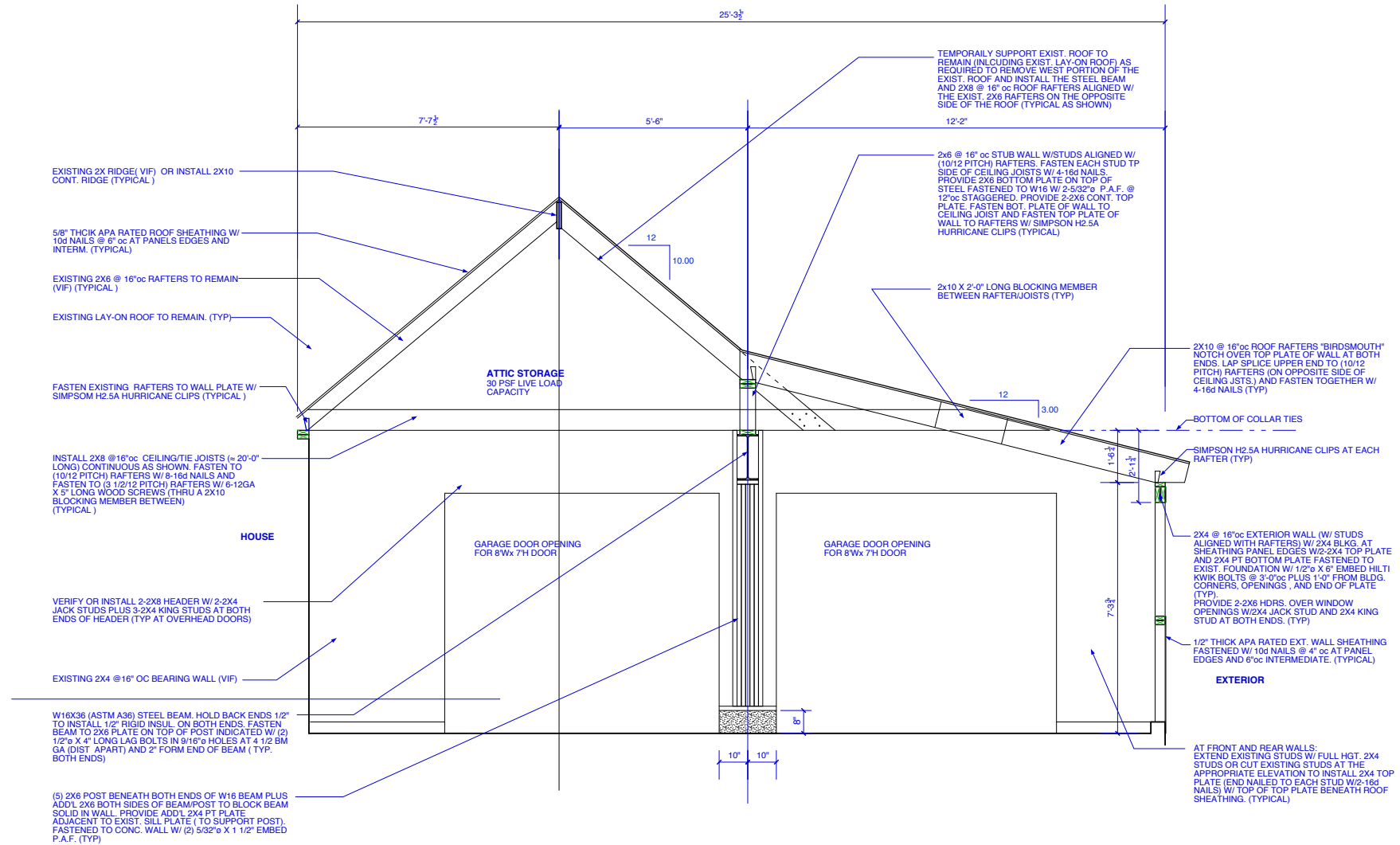
1 GARAGE - NEW ROOF SECTION SCALE: 1/2" = 1'-0"
