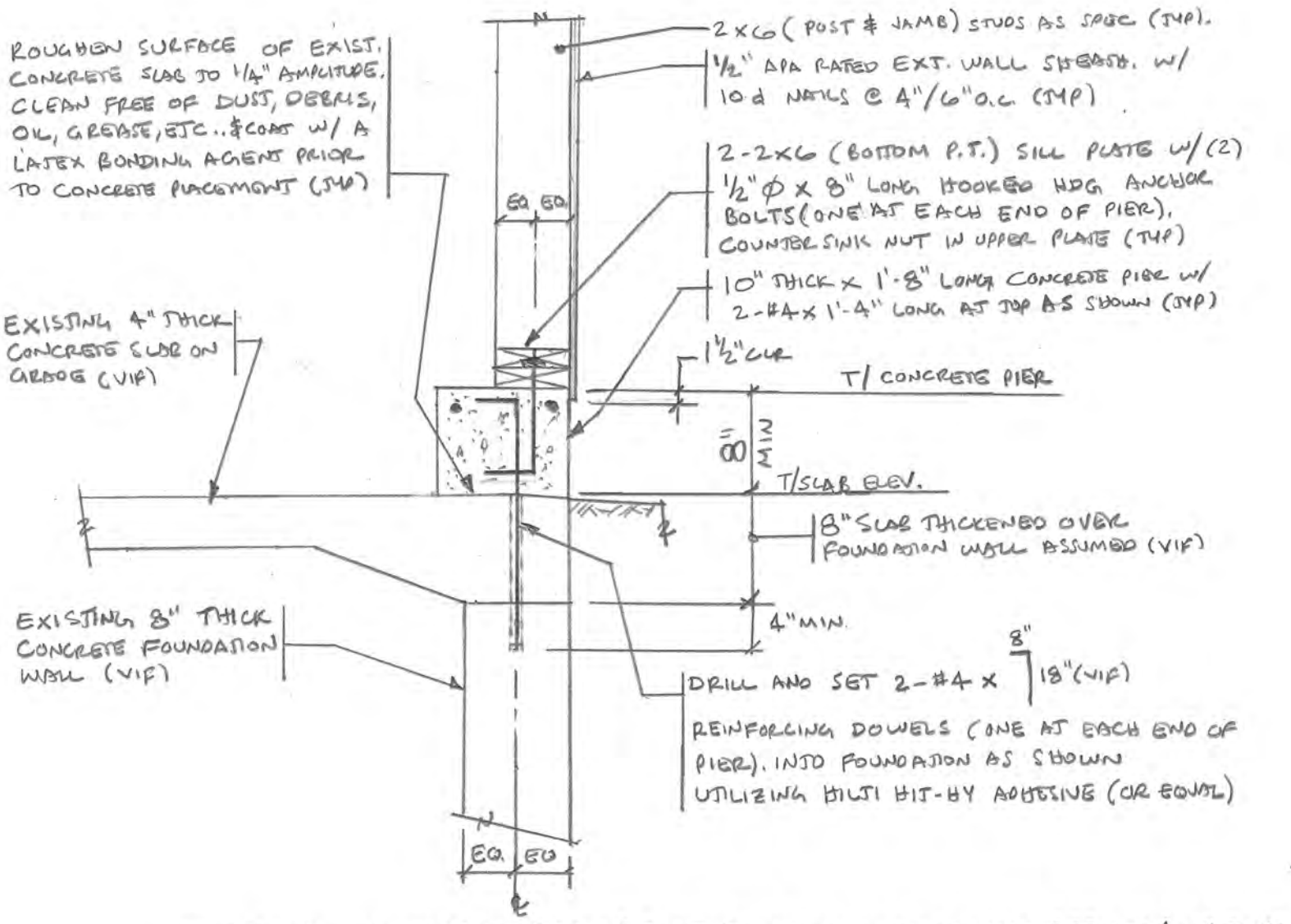
SECTION - FOUNDATION RETROFIT AT FRONT WALL OF GARAGE BETWEEN O.H. DOORS.
