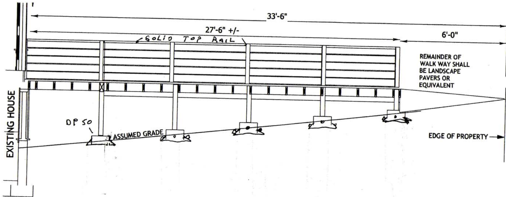
ELEVATION CROSS SECTION
