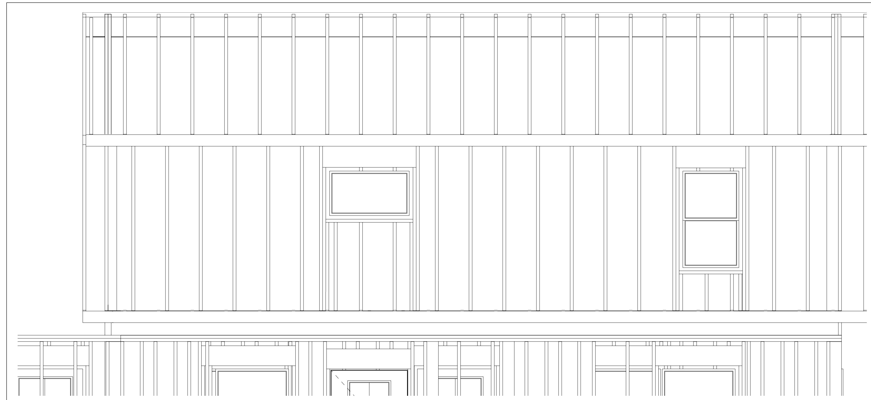
PROPOSED DORMER EAVE FRAMING SCALE: 1/2" = 1'-0"
