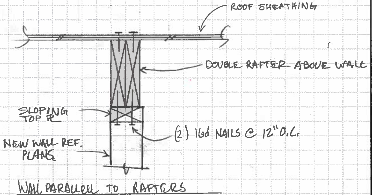
② TOP OF NEW WALL DETAIL
