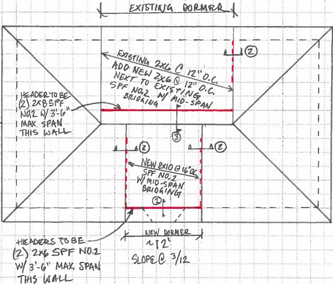
ROOF PLAN 1/8" = 1'-0"
