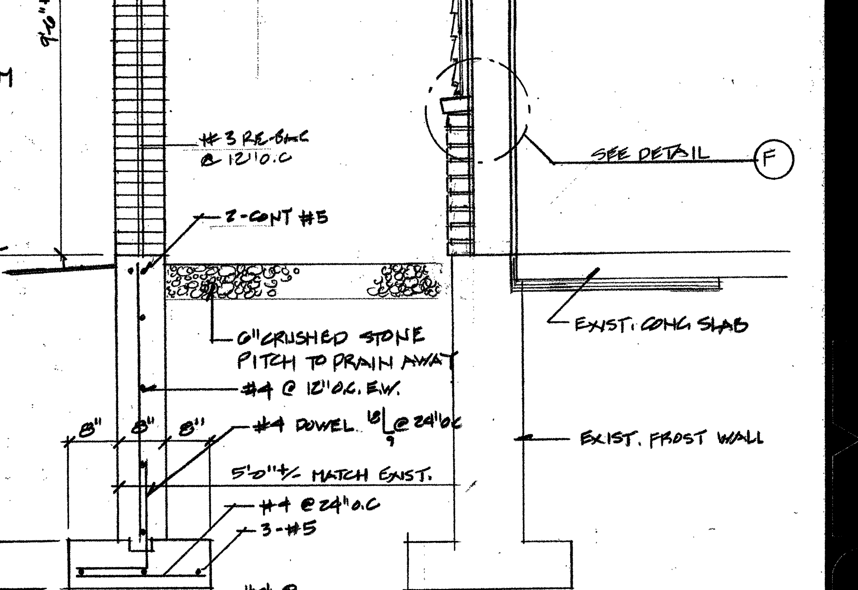
WALL SECTION 3/4" = 1'-0"
