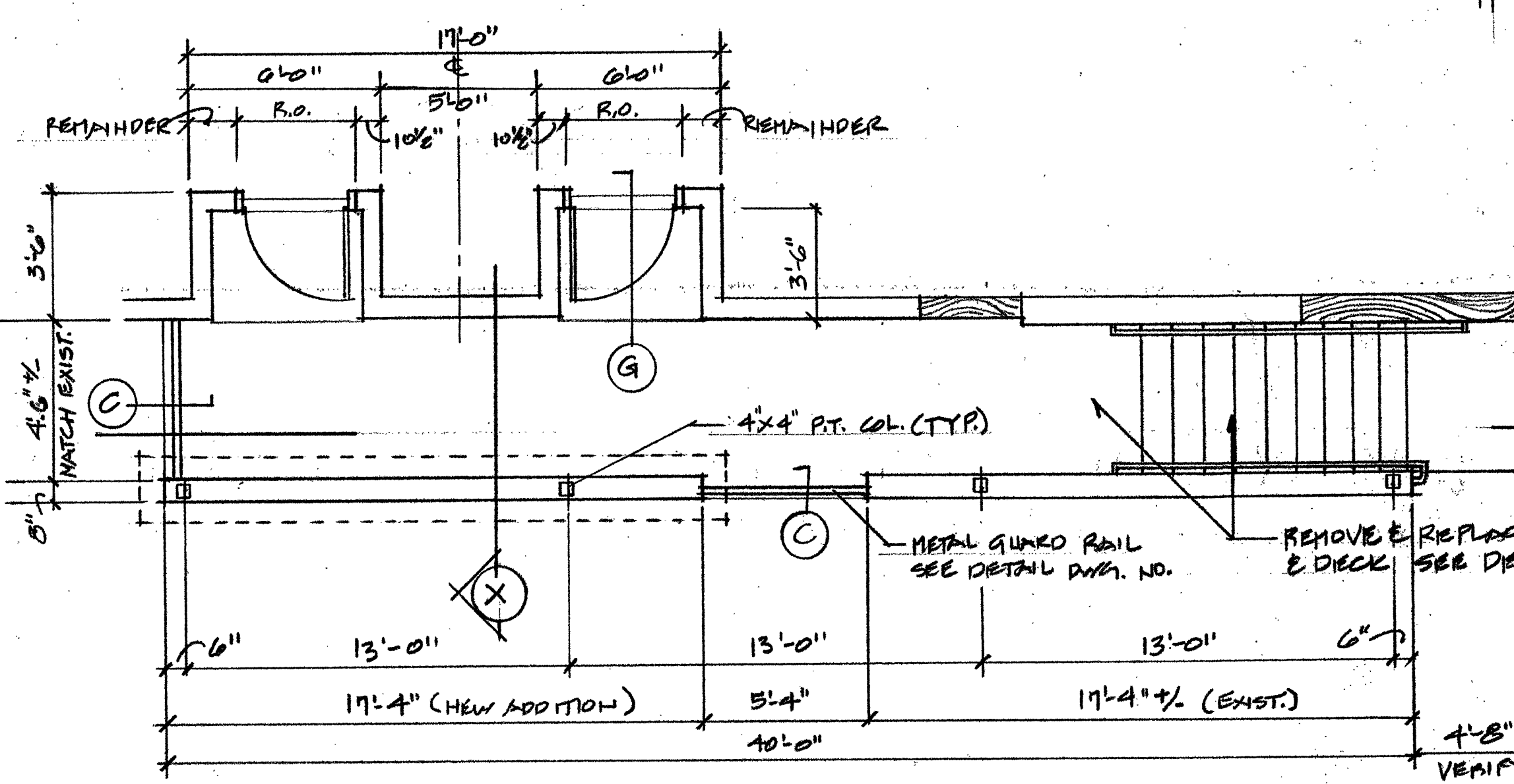
COVERED EGRESS DECK 1/2" = 1'-0"
