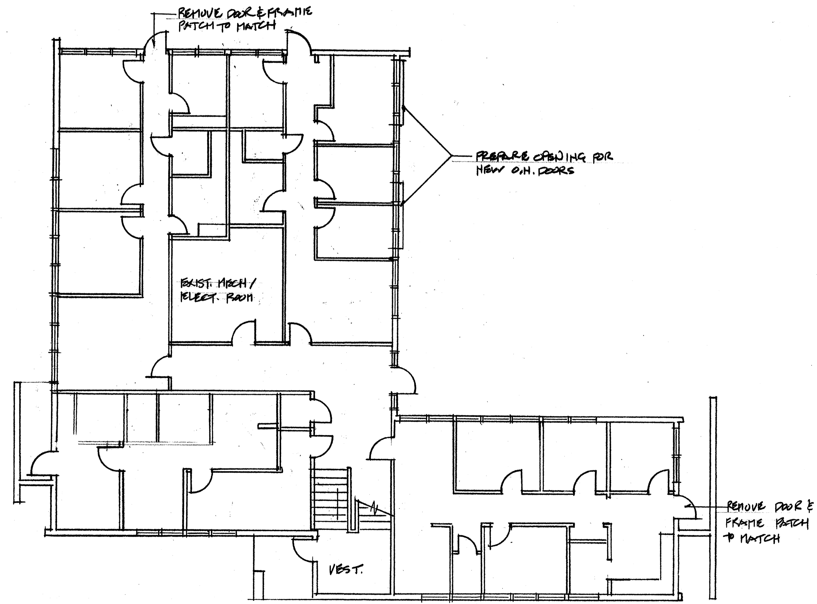
LOWER LEVEL REMOVAL PLAN 1/8"=1'-0"
