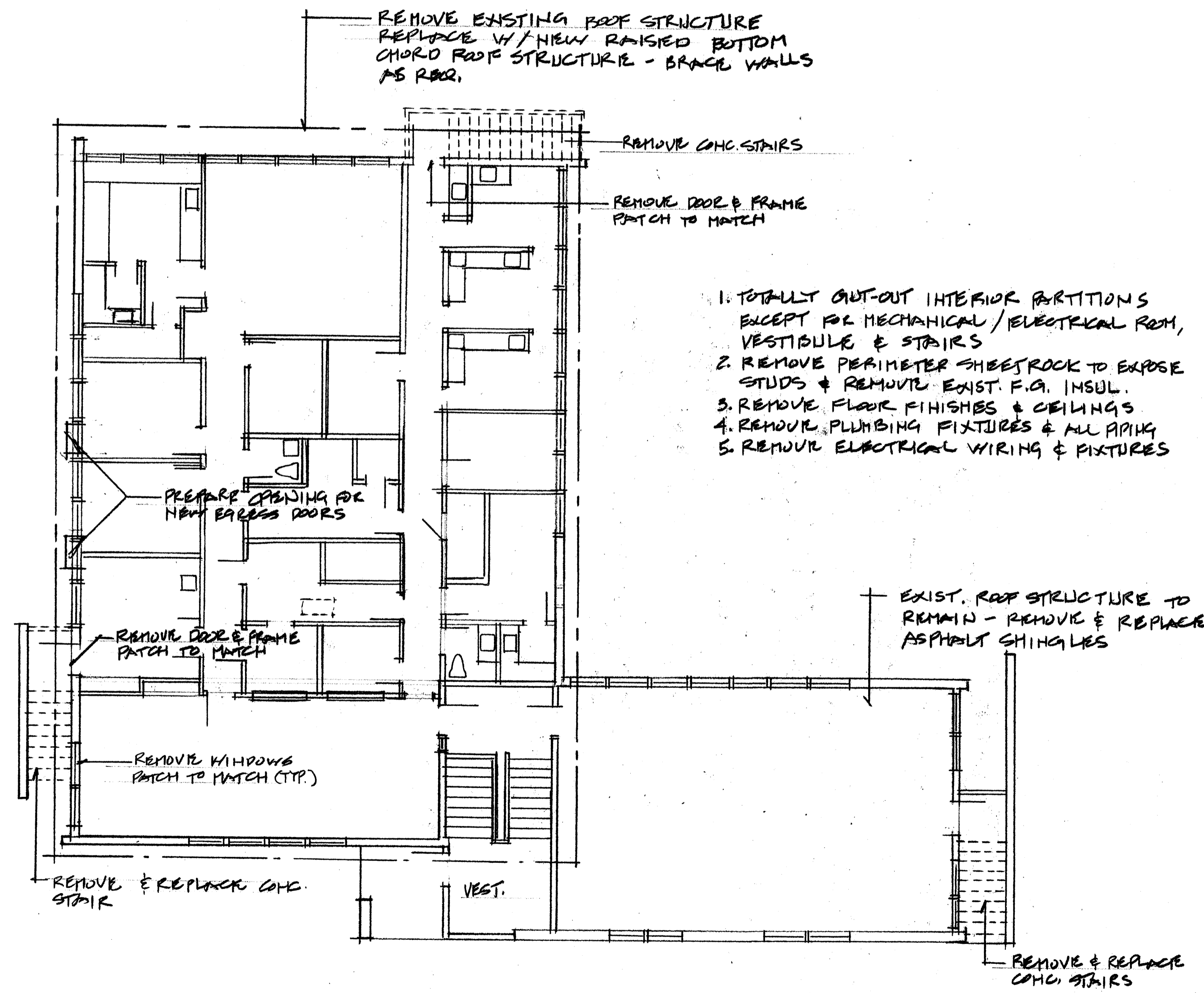
UPPER LEVEL REMOVAL PLAN 1/8"=1'-0"
