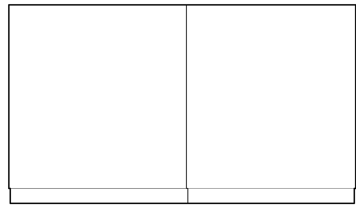
7 BED #3 ELEV. A1.3 3/8" = 1'-0"
