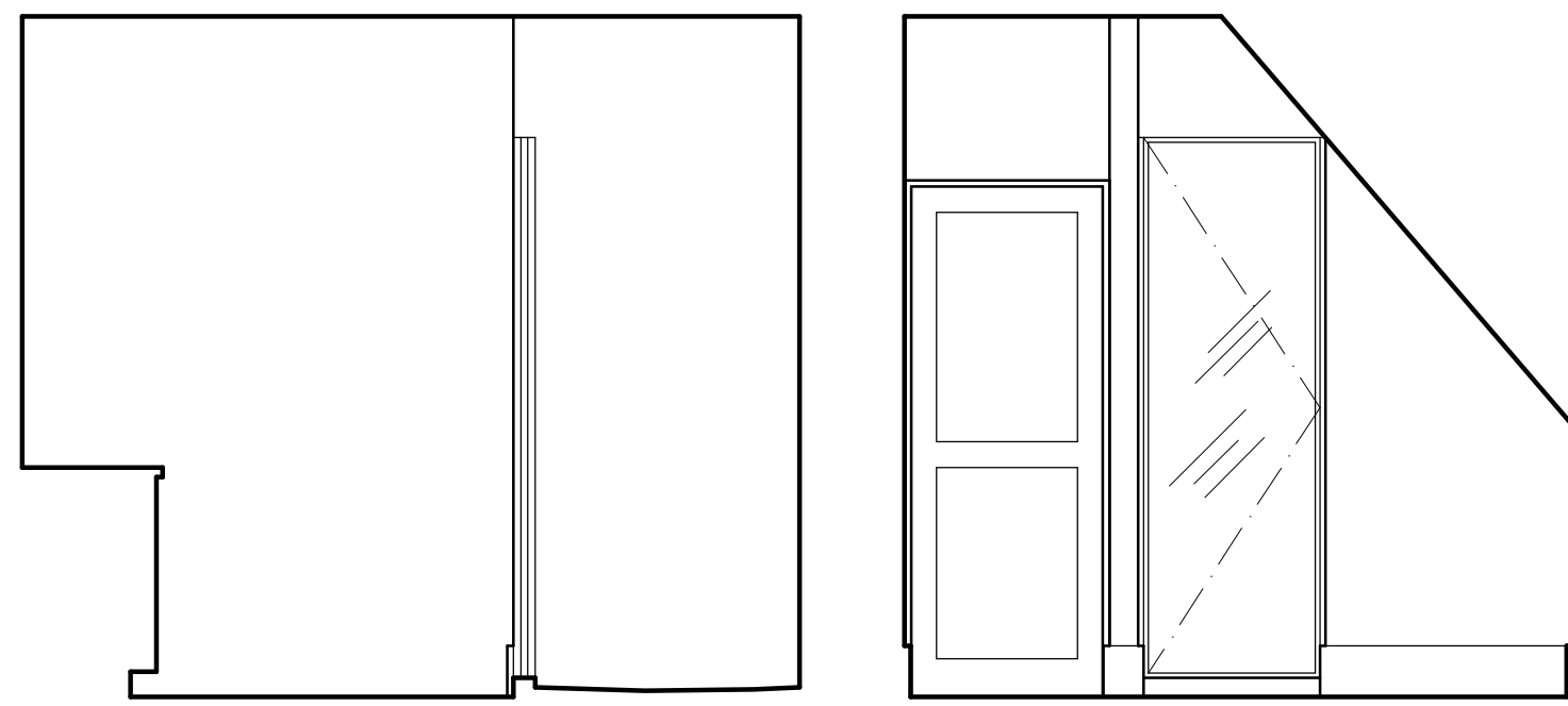
1 MASTER BATH ELEV. A1.3 3/8" = 1'-0"
