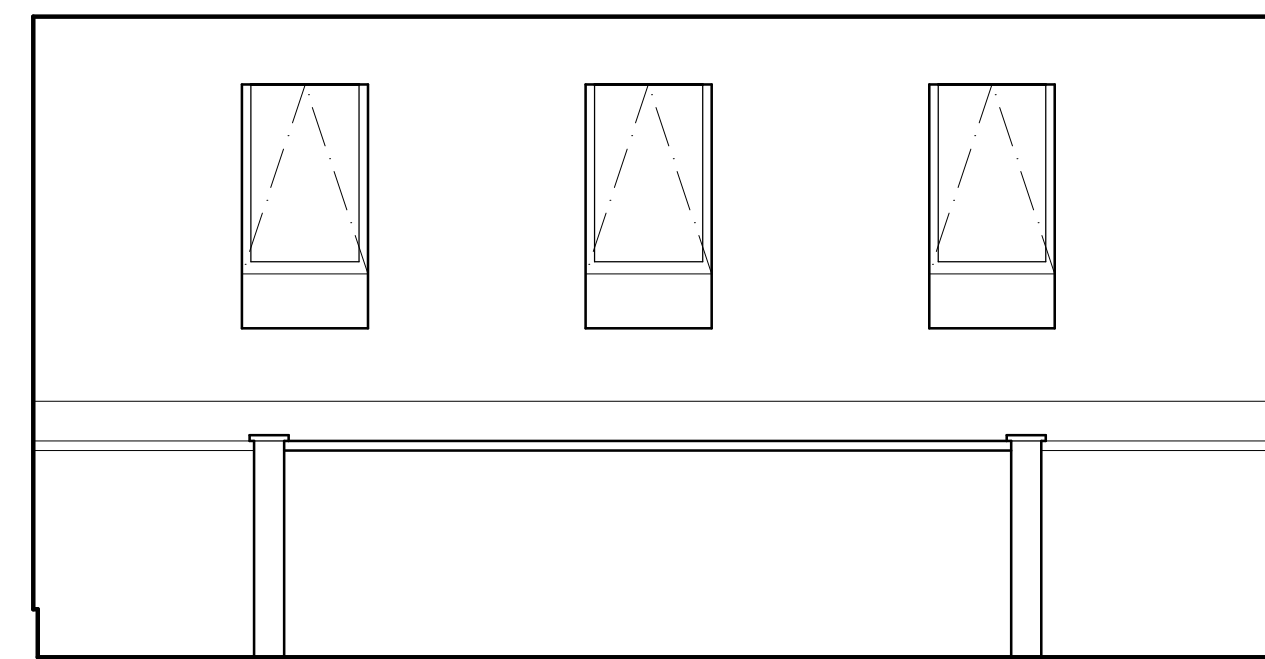
5 UPPER HALL ELEV. A1.3 3/8" = 1'-0"
