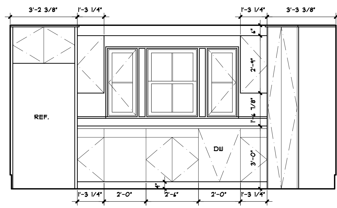
1 KITCHEN ELEVS. A1.2 3/8" = 1'-0"
