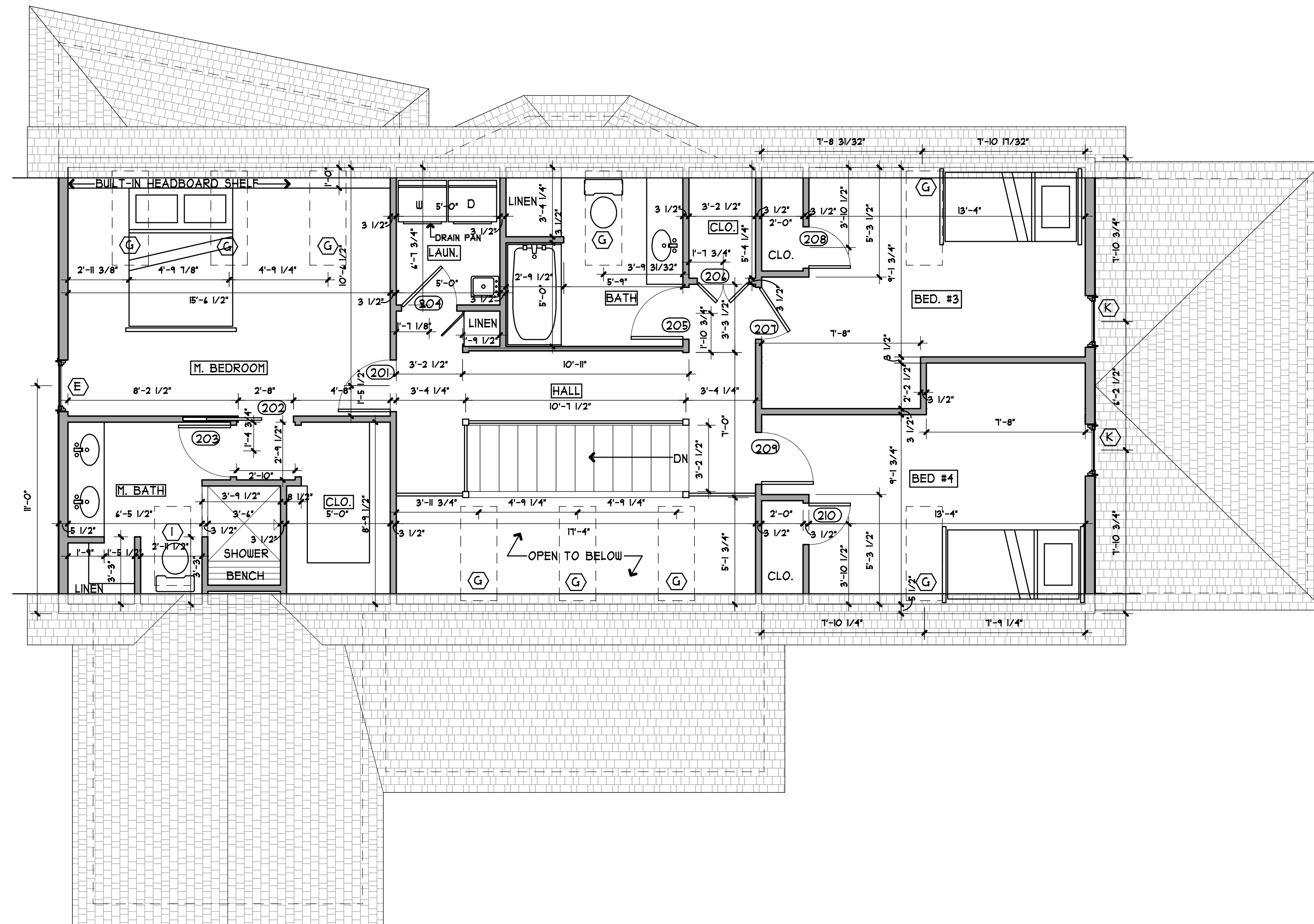
1 SECOND FLOOR PLAN 944.20 SQ. FT. CONDITIONED SPACE A3.3 1/4" = 1'-0"
