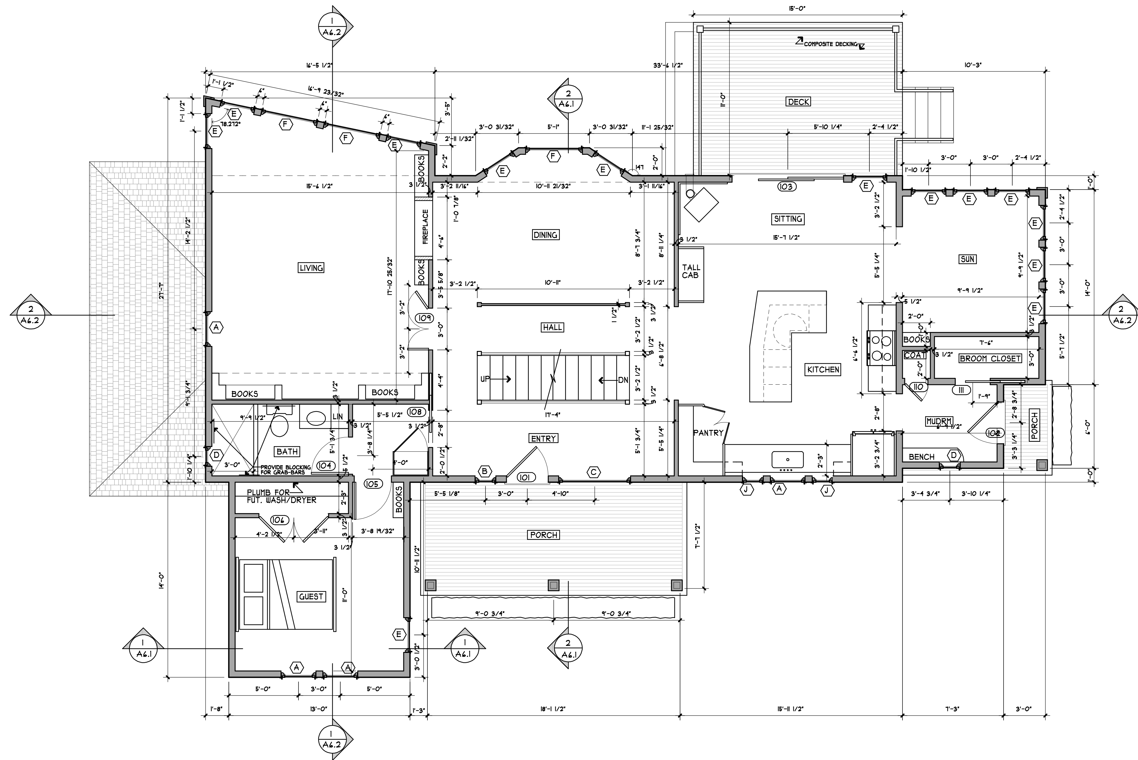
1 FIRST FLOOR PLAN 1549.61 SQ. FT. CONDITIONED SPACE A3.2 1/4" = 1'-0"
