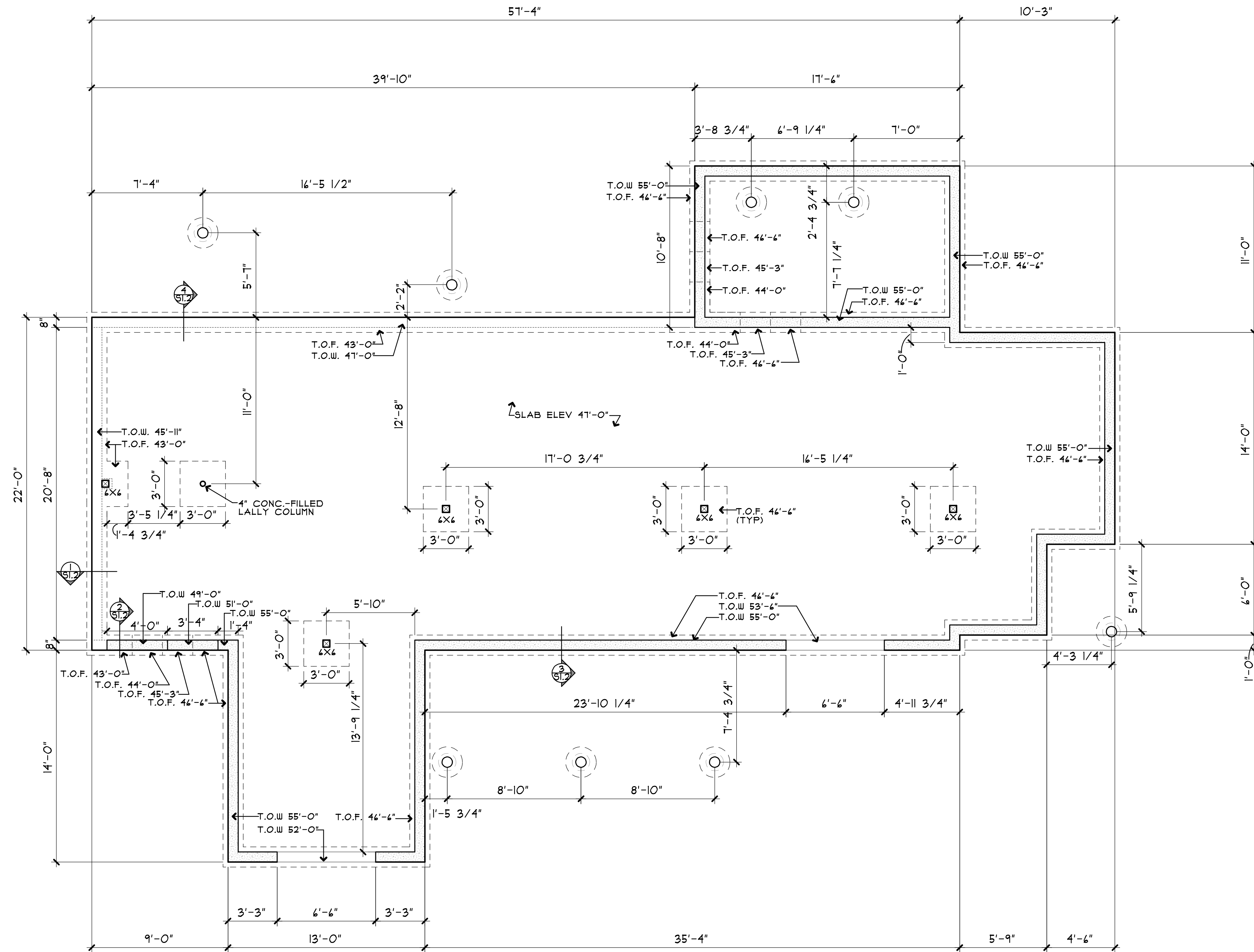
1 FOUNDATION PLAN S.I.1 1/4" = 1'-0"
