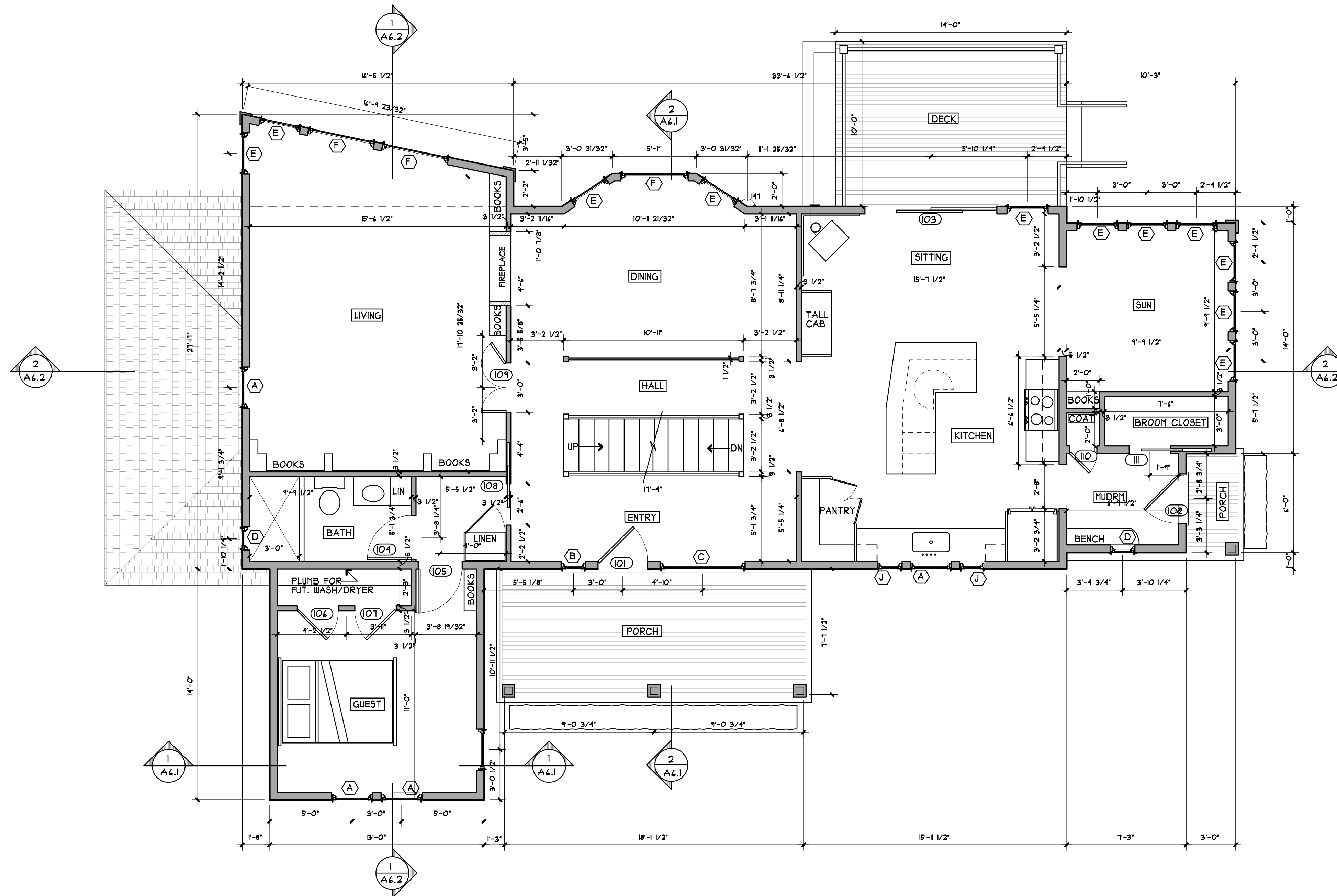
1 FIRST FLOOR PLAN A3.2 1/4" = 1'-0"
