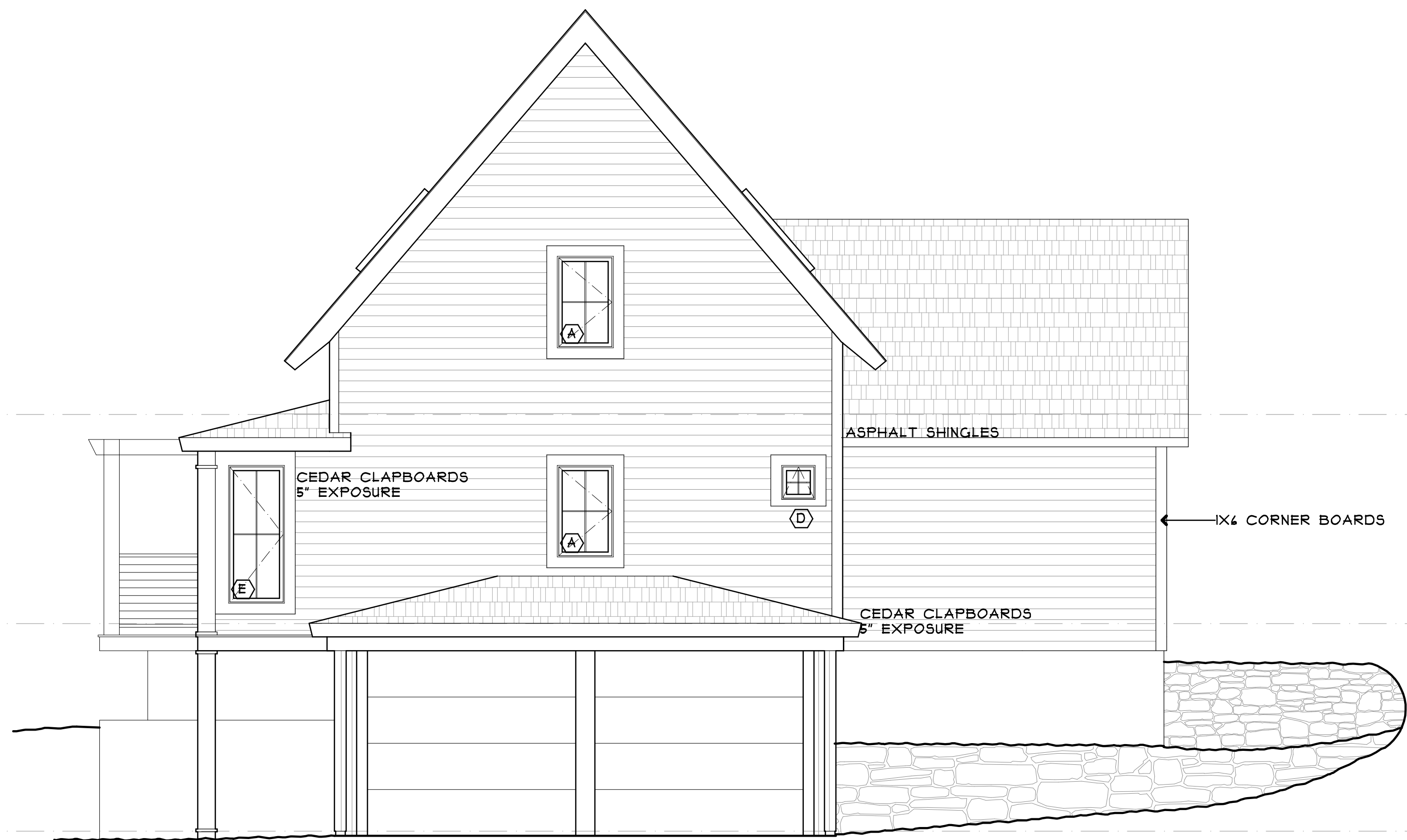
1 NORTHEAST ELEVATION 1/4" = 1'-0"
