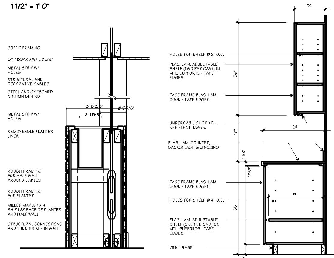
CABINET SECTION
