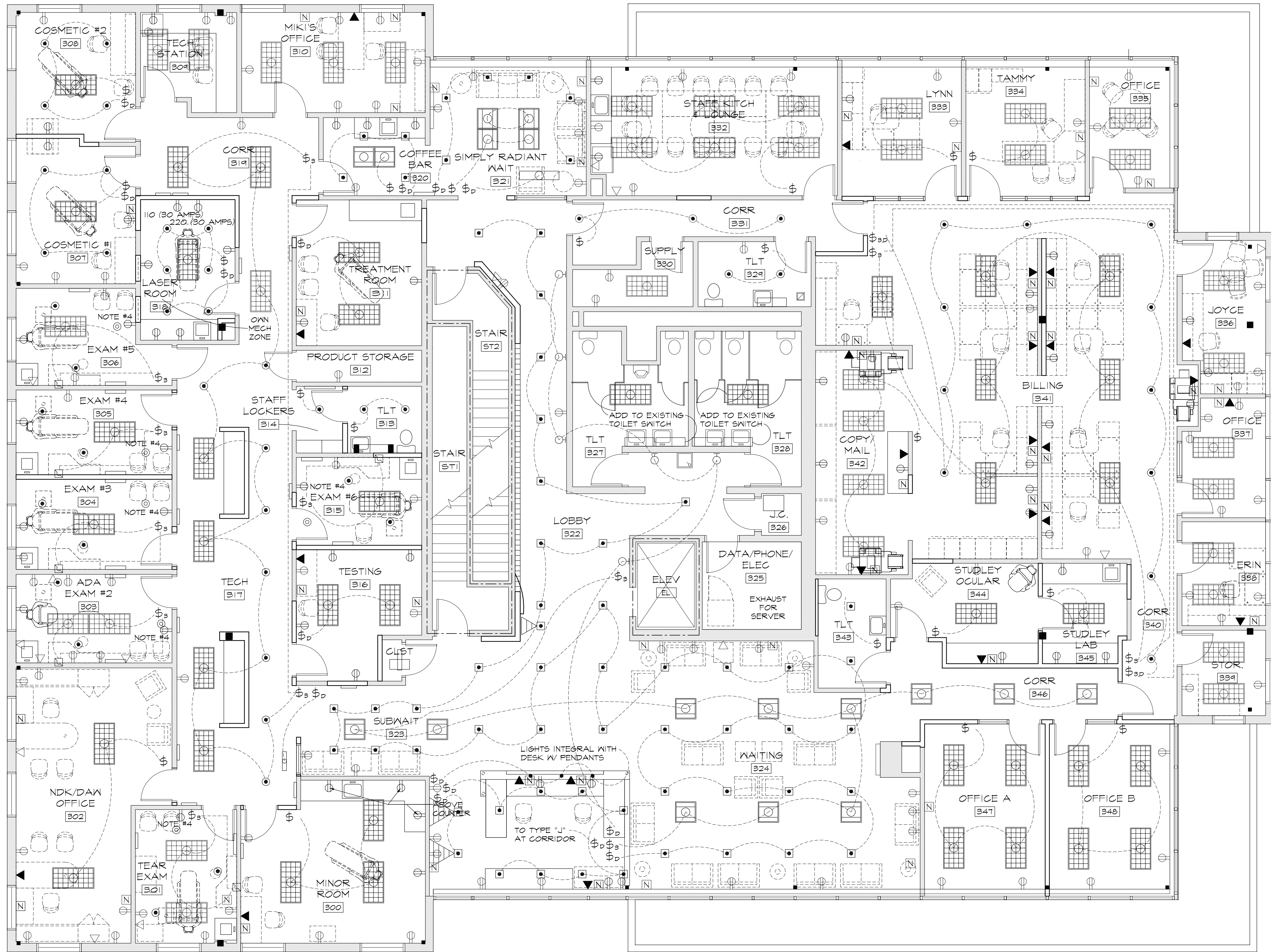
1 POWER / SWITCHING PLAN 3/16"=1'-0"
