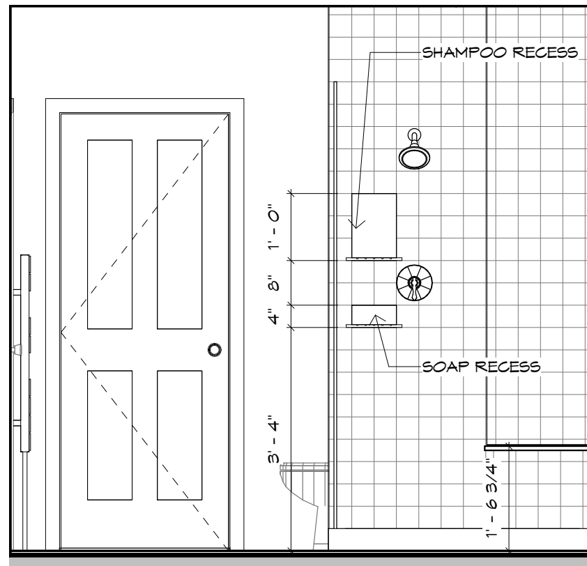
2 BATHROOM INT ELEV B - SUITE B A501 1/2" = 1'-0"
