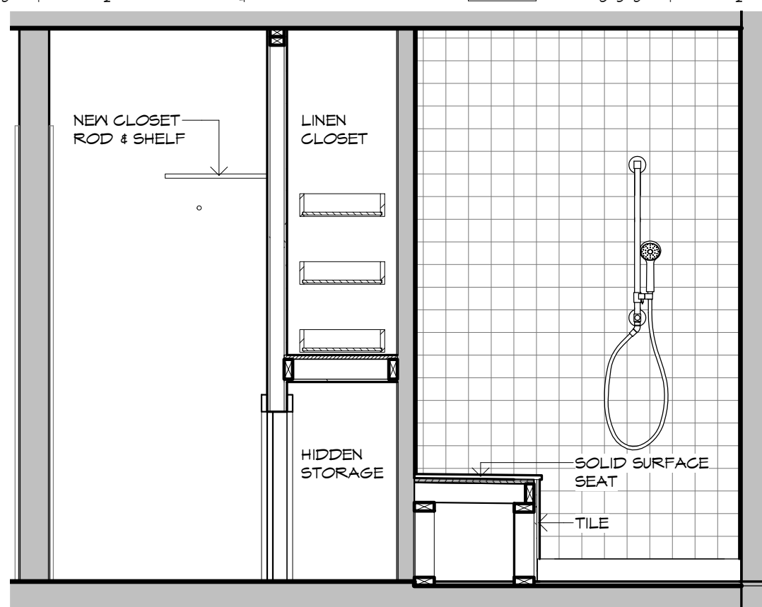
2 BATHROOM INT ELEV B - SUITE B A501 1/2" = 1'-0"
