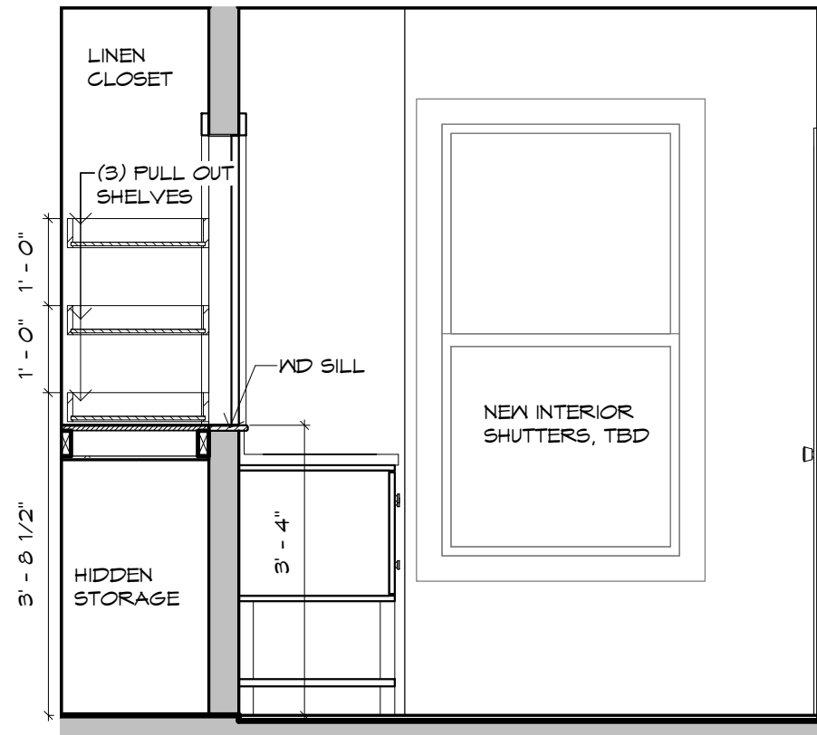
3 BATHROOM INT ELEV C - SUITE B A501 1/2" = 1'-0"
