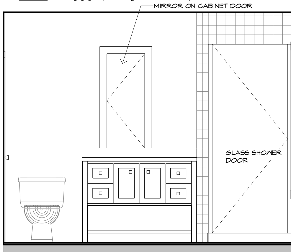
1 BATHROOM INT ELEV A - SUITE B A501 1/2" = 1'-0"
