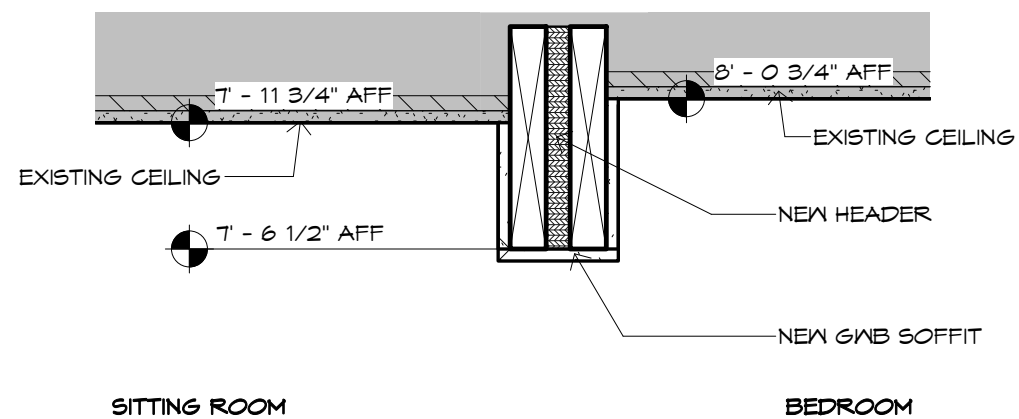
3 SOFFIT @ FORMER WALL A400 1 1/2" 0" 1" 2" 4" 8" 1' 1'-4"
