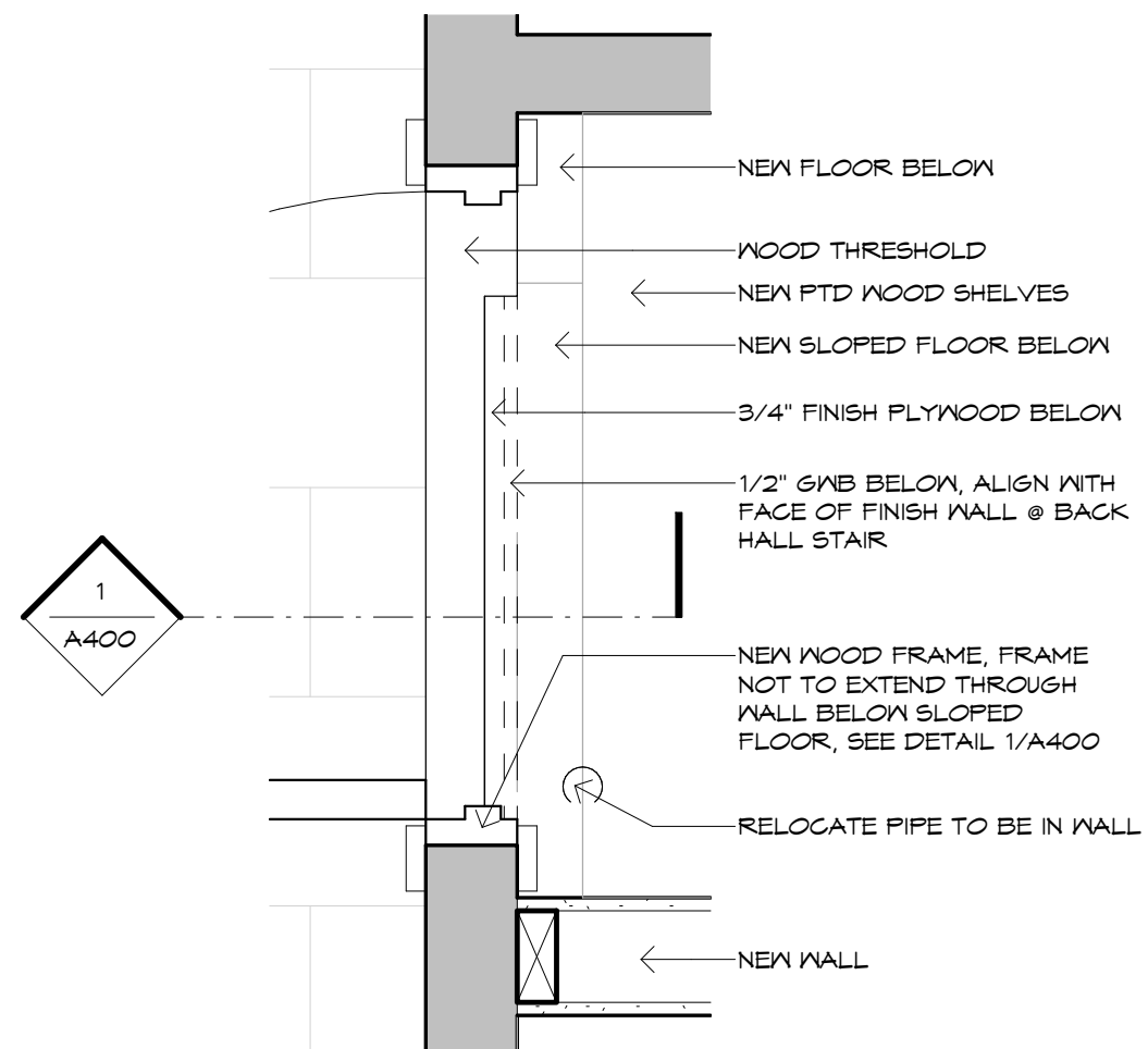
2 DOOR DETAIL @ SUITE B BATHROOM CLOSET A400 1 1/2" 0" 1" 2" 4" 8" 1' 1'-4"
