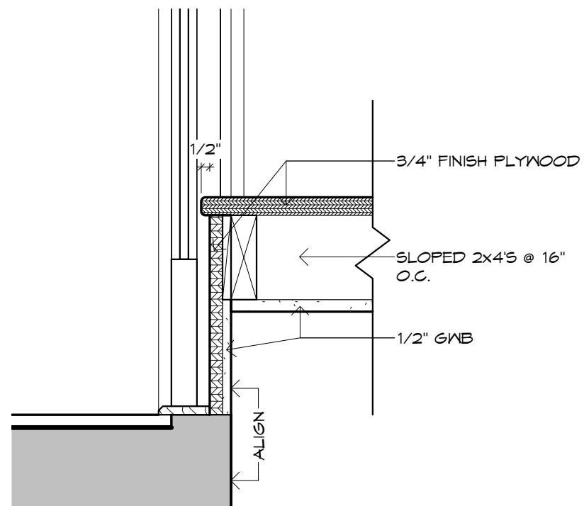
1 FLOOR DETAIL @ SUITE B BATHROOM CLOSET A400 1 1/2" 0" 1" 2" 4" 8" 1' 1'-4"
