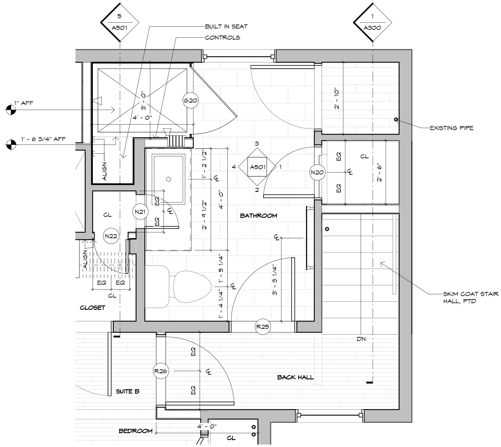
1 ENLARGED PLAN - SUITE B BATHROOM A113 1/2" = 1'-0"
