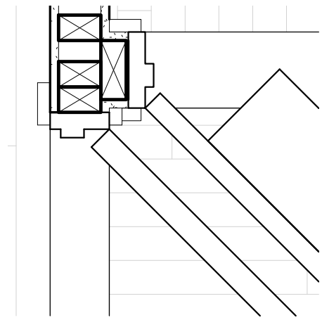
2 DOOR DETAIL @ CORNER A112 1 1/2" = 1'-0"
