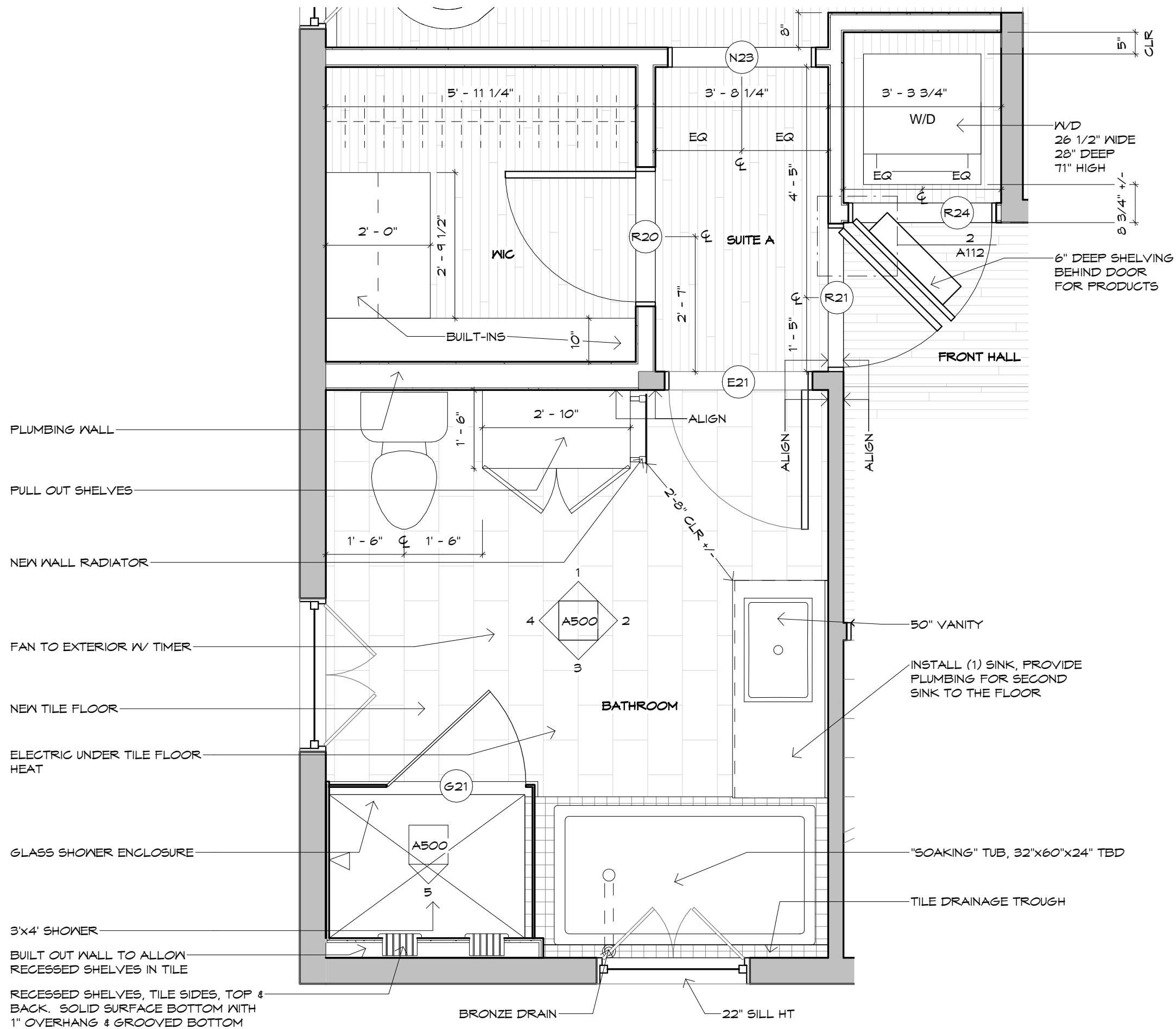
1 ENLARGED PLAN - SUITE A BATHROOM A112 1/2" = 1'-0"
