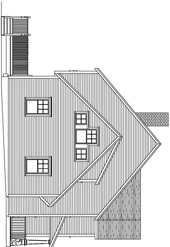
LEFT ELEVATION SCALE 3/8" = 1'-0"
