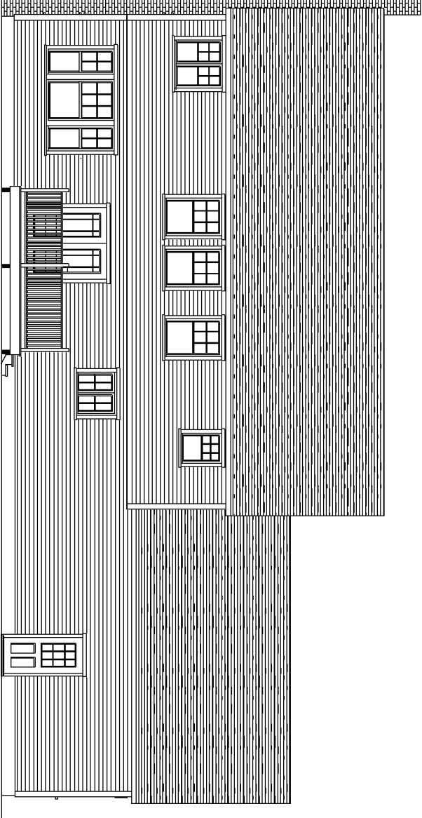
REAR ELEVATION SCALE 3/8" = 1'-0"
