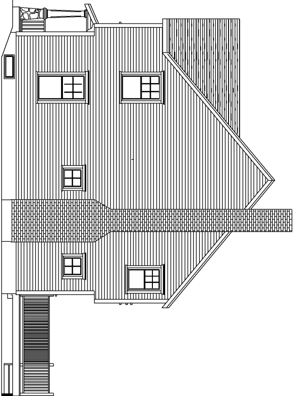
RIGHT ELEVATION SCALE 3/8" = 1'-0"
