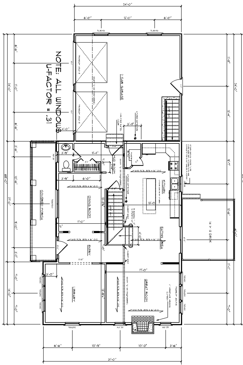
MAIN FLOOR PLAN SCALE 1/8" = 1'-0"
