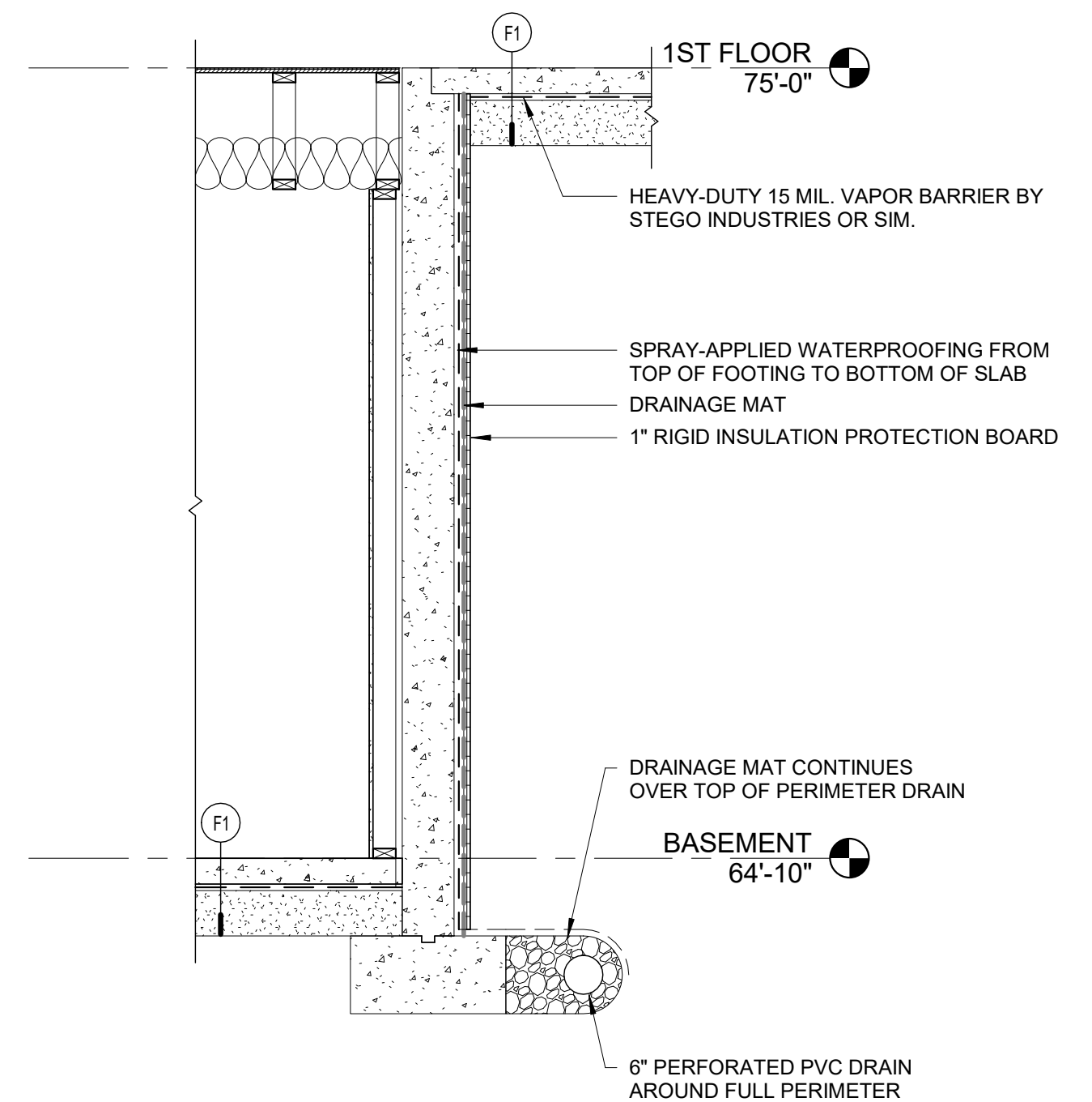
2 FOUNDATION WATERPROOFING 1/2" = 1'-0"
