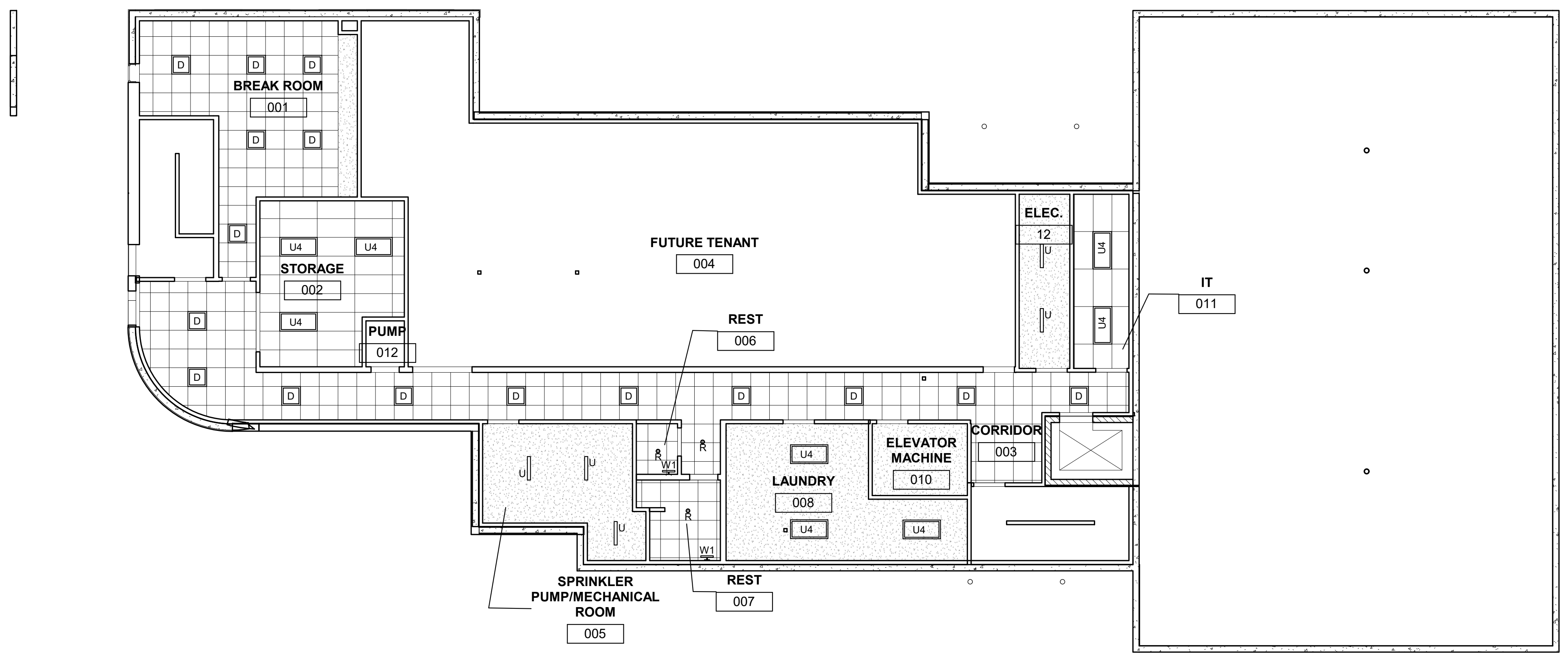
2 BASEMENT CEILING PLAN 1/8" = 1'-0"
