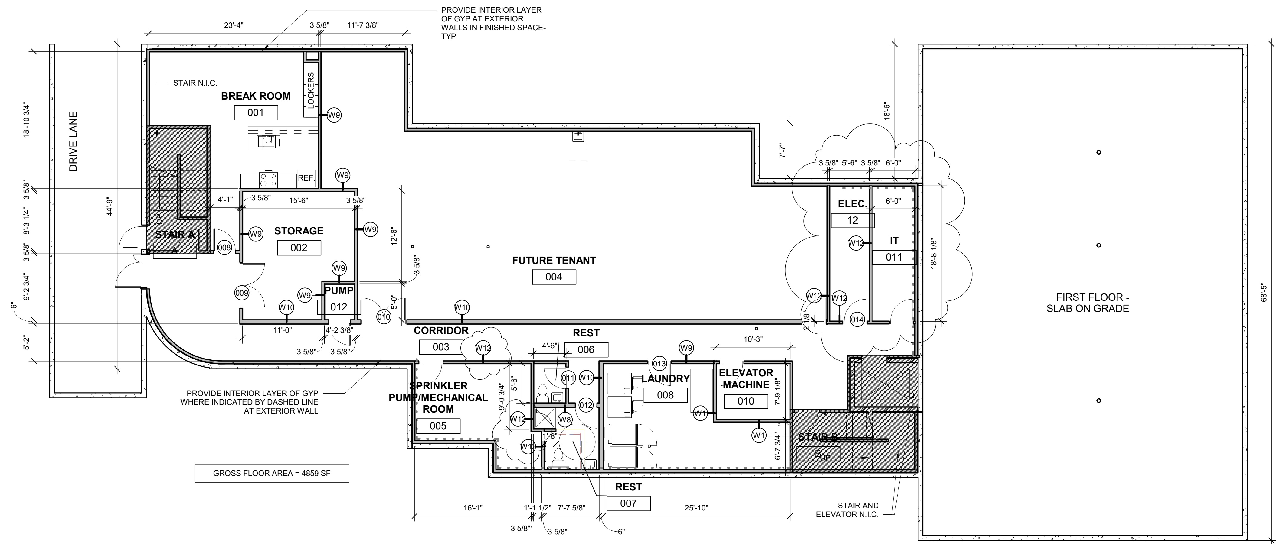
1 BASEMENT FIT OUT 1/8" = 1'-0"
