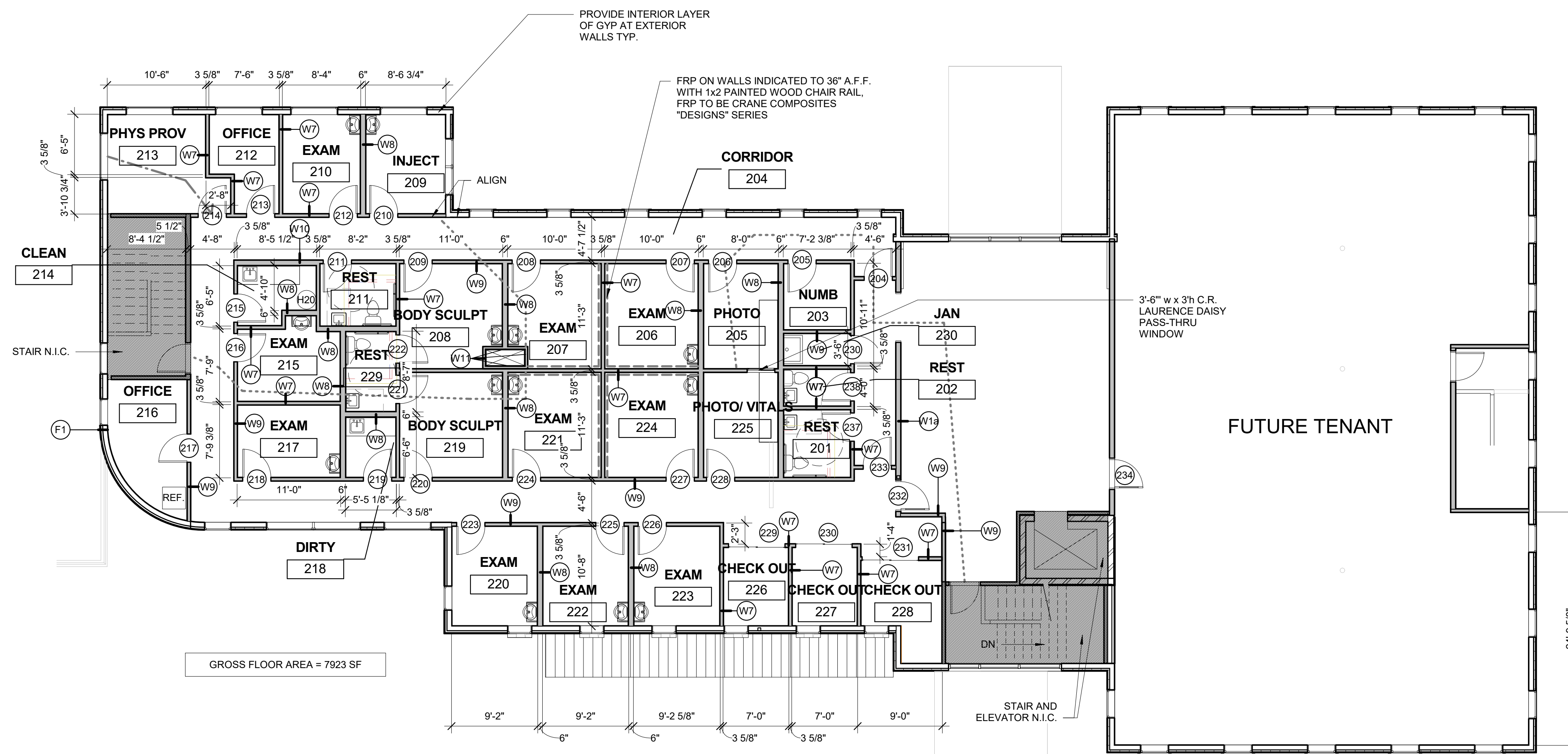
1 | 2ND FLOOR -FIT OUT 1/8" = 1'-0"
