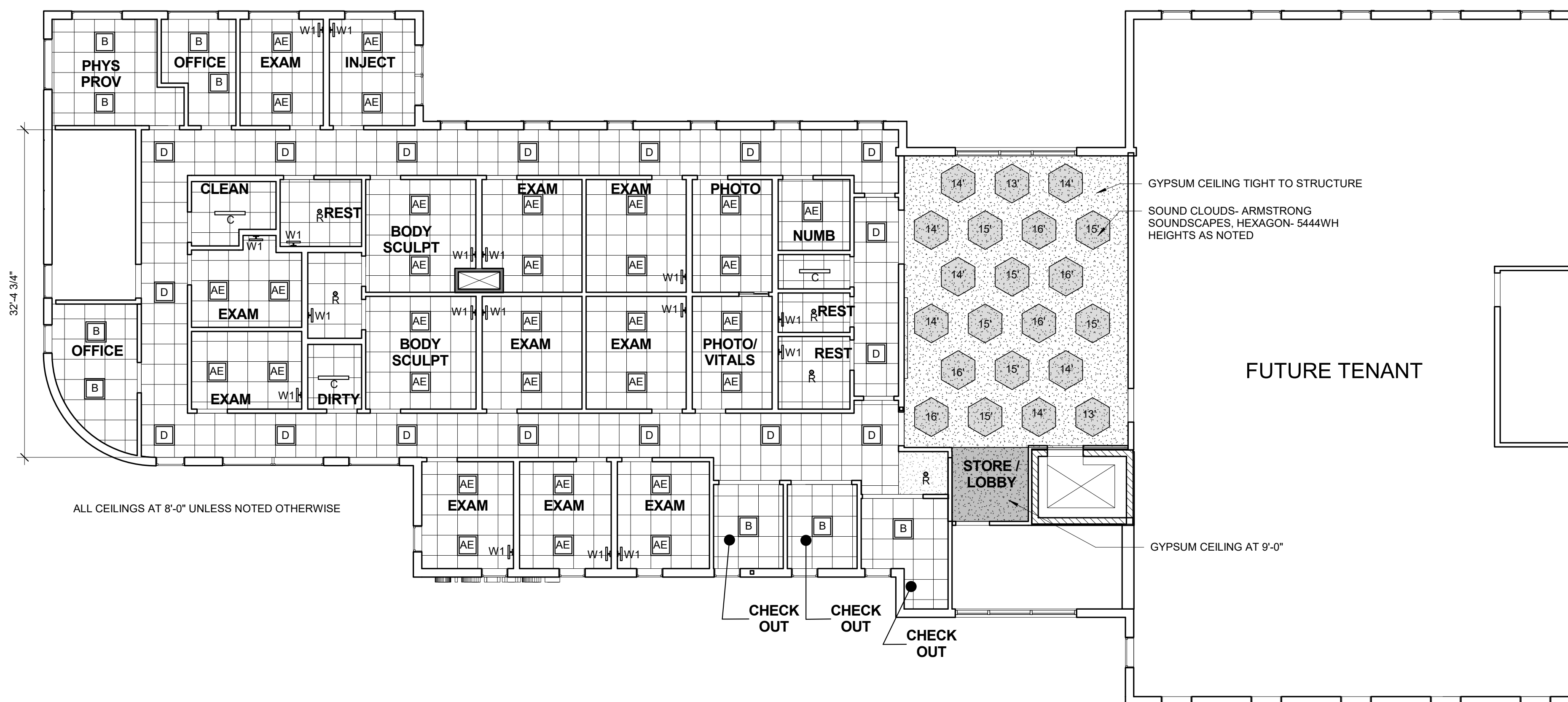
1 | 2ND FLOOR -FIT OUT 1/8" = 1'-0"
