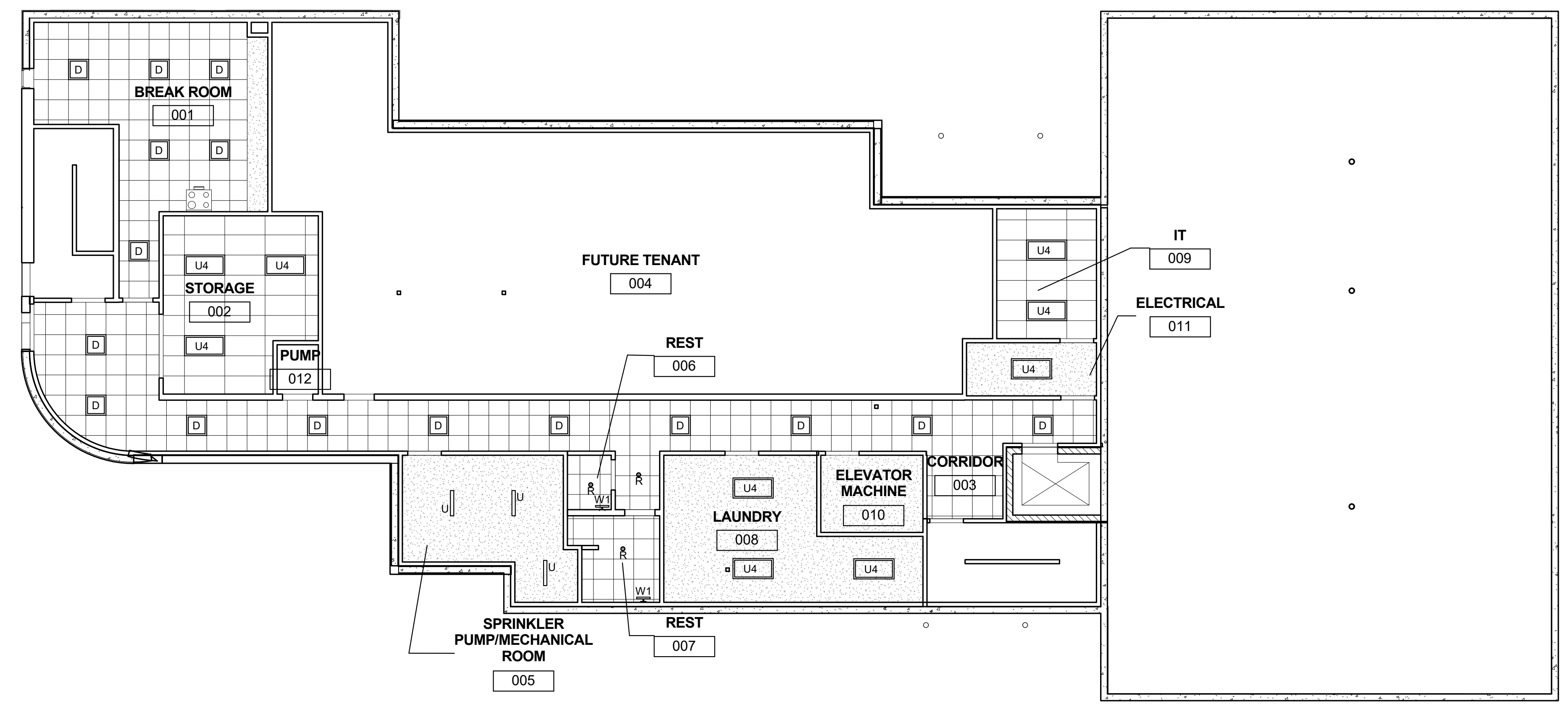
2 BASEMENT CEILING PLAN 1/8" = 1'-0"
