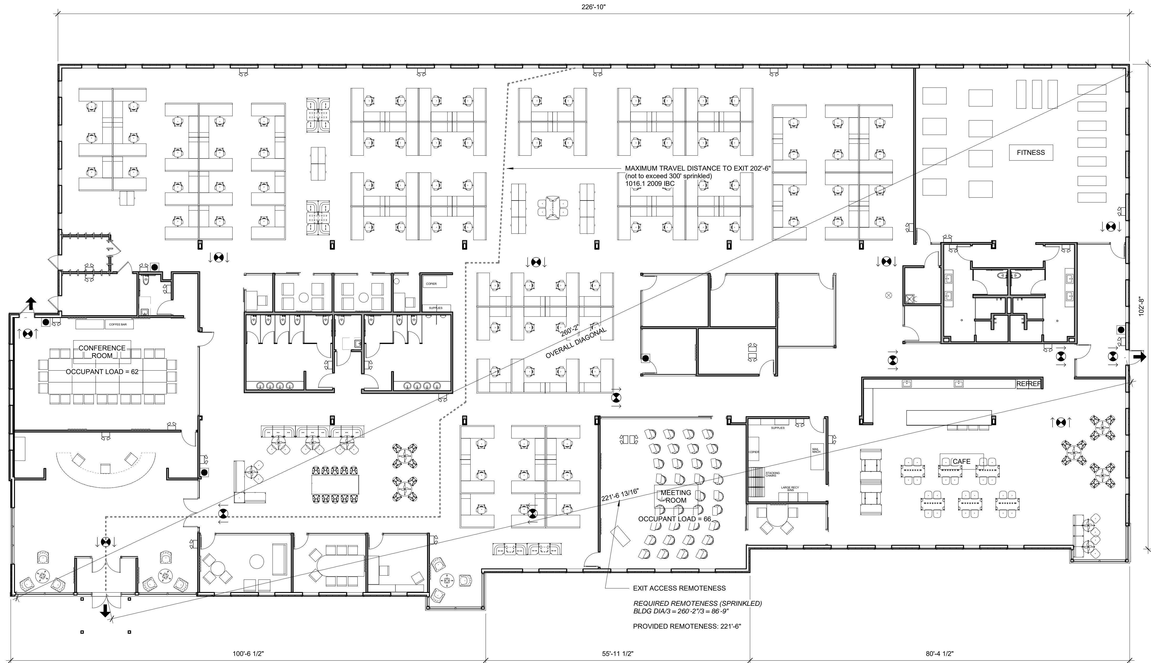
1 | 1ST FLOOR - LIFE SAFETY 3/32" = 1'-0"
