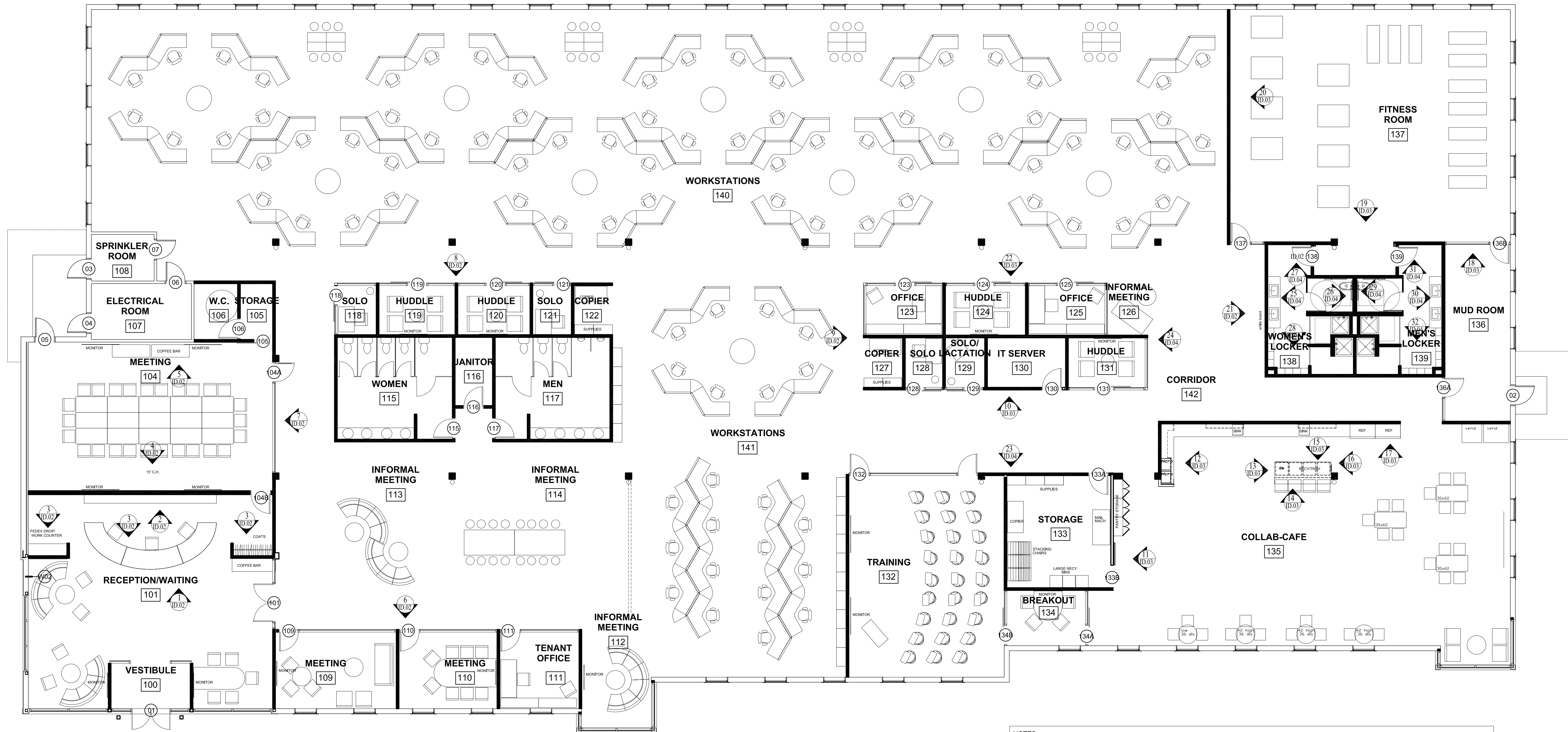
1 | FURNITURE PLAN 1/8" = 1'-0"
