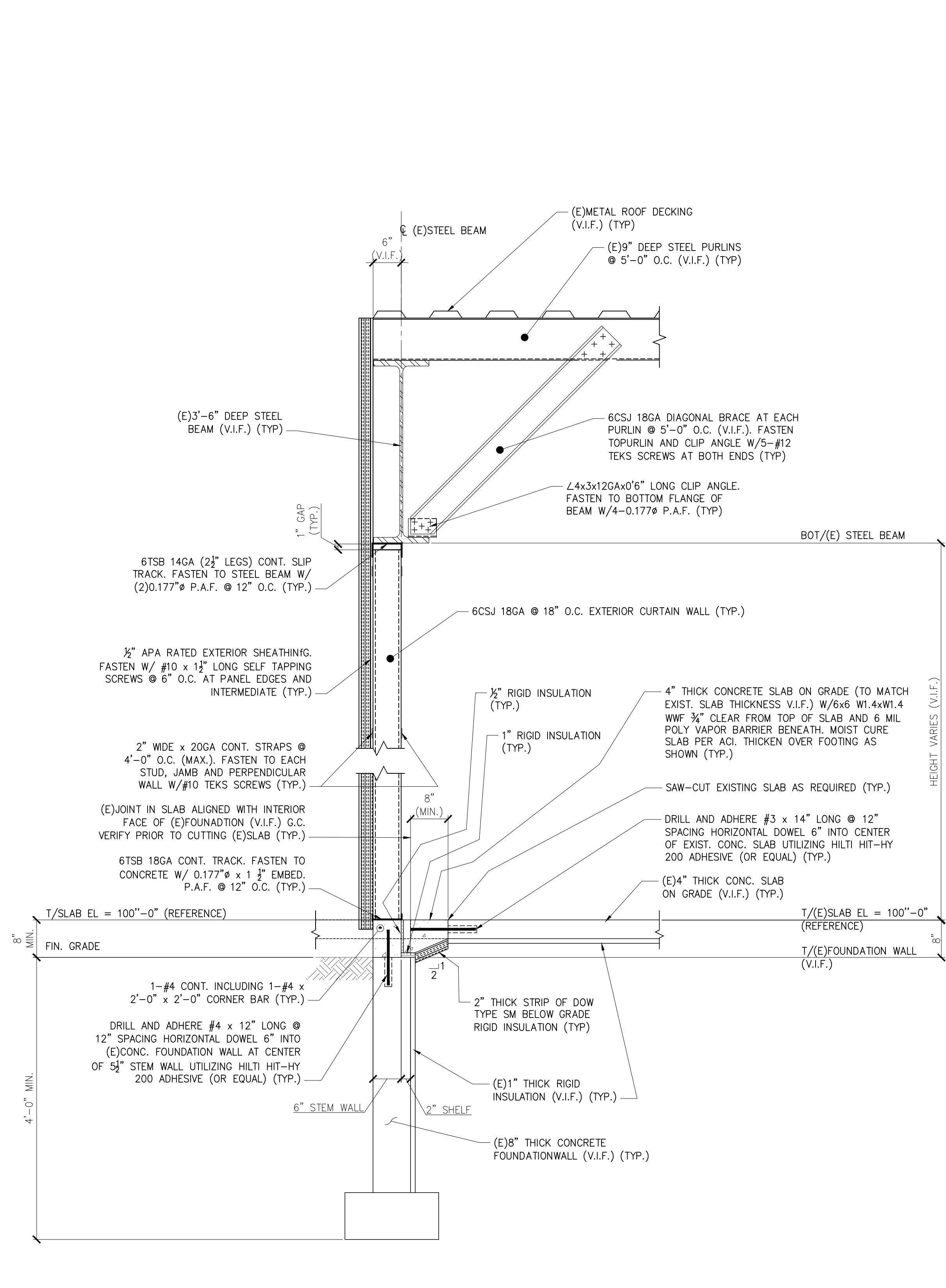
SECTION 1 3/4" = 1'-0" S1.0 S1.1
