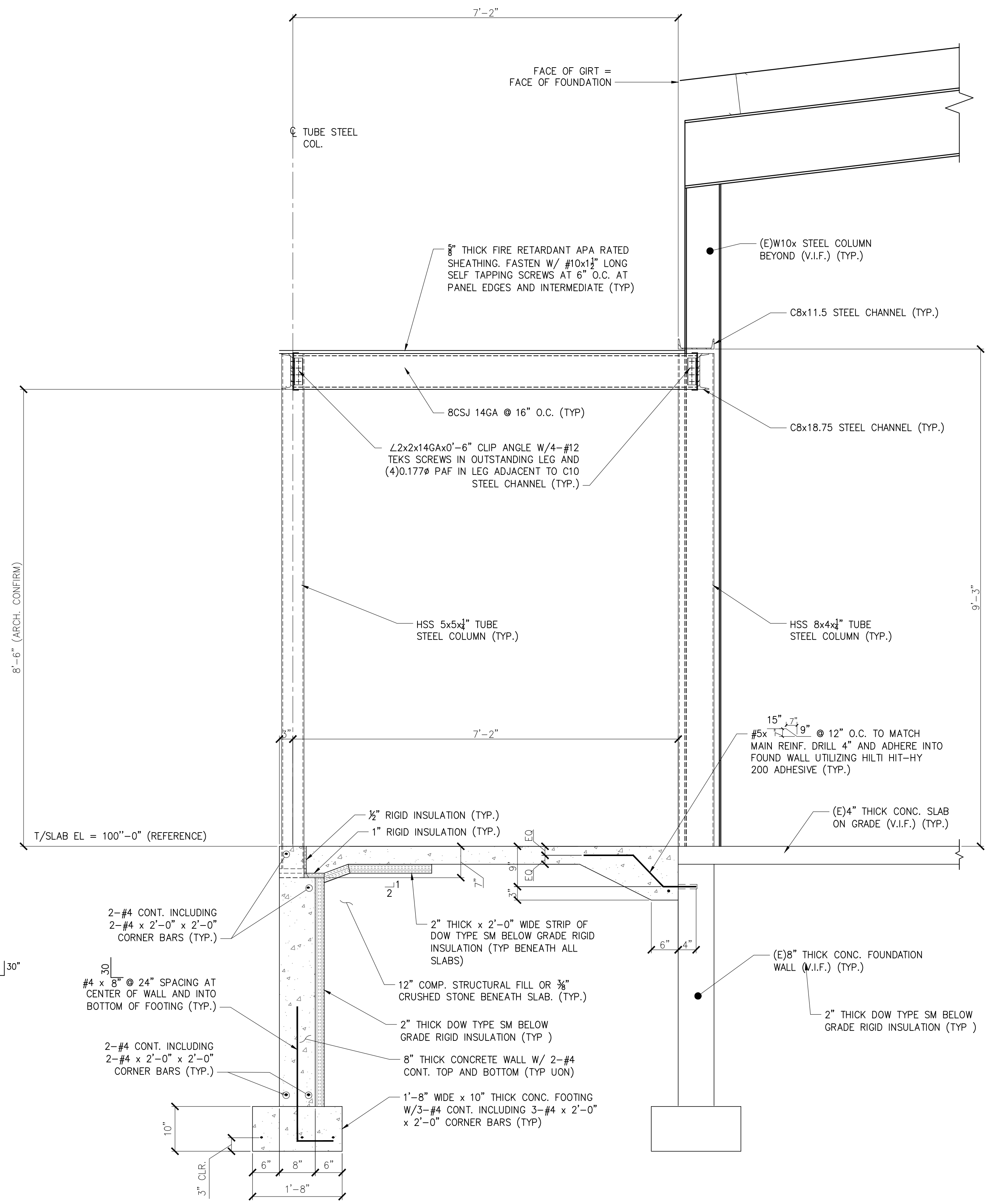
SECTION 6 3/4" = 1'-0" S1.1
