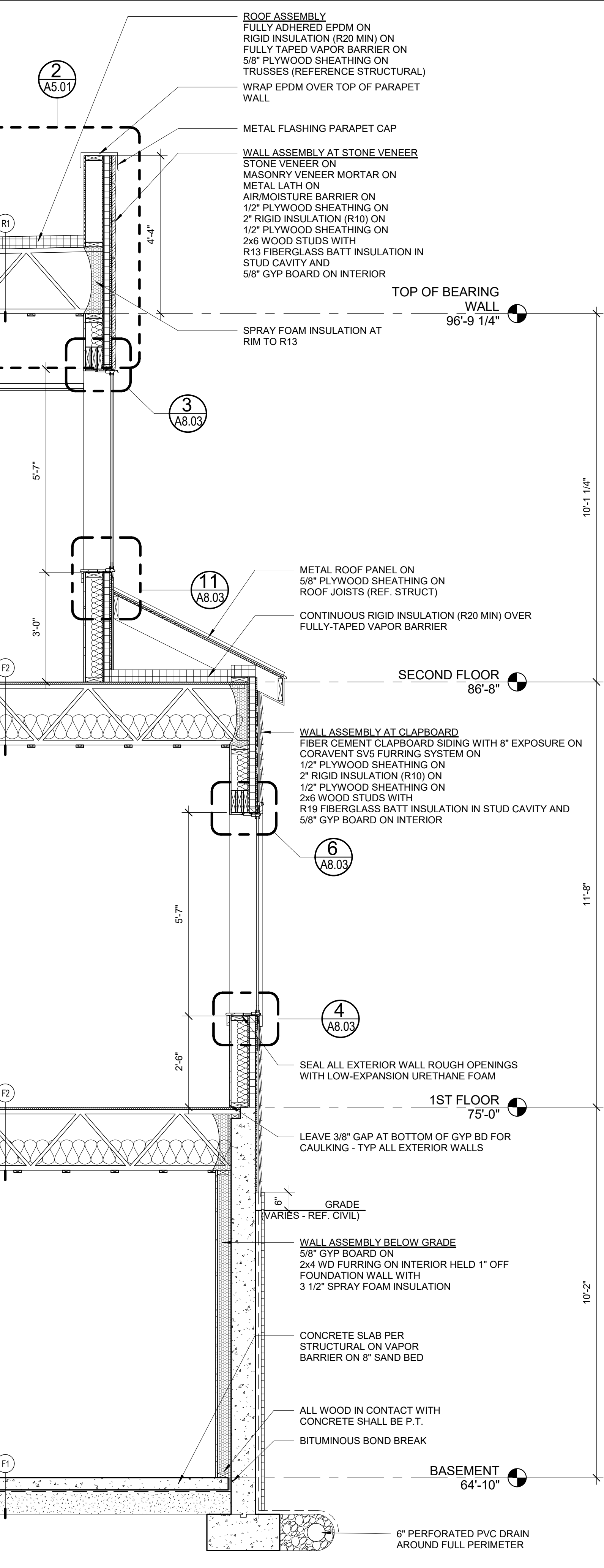
1 | WALL SECTION 1 1/2" = 1'-0"
