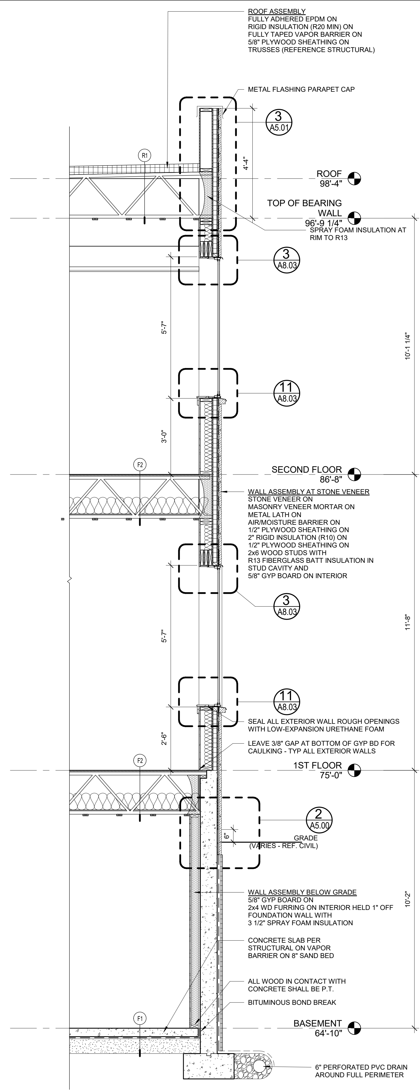
4 | WALL SECTION AT STONE VENEER 1/2" = 1'-0"
