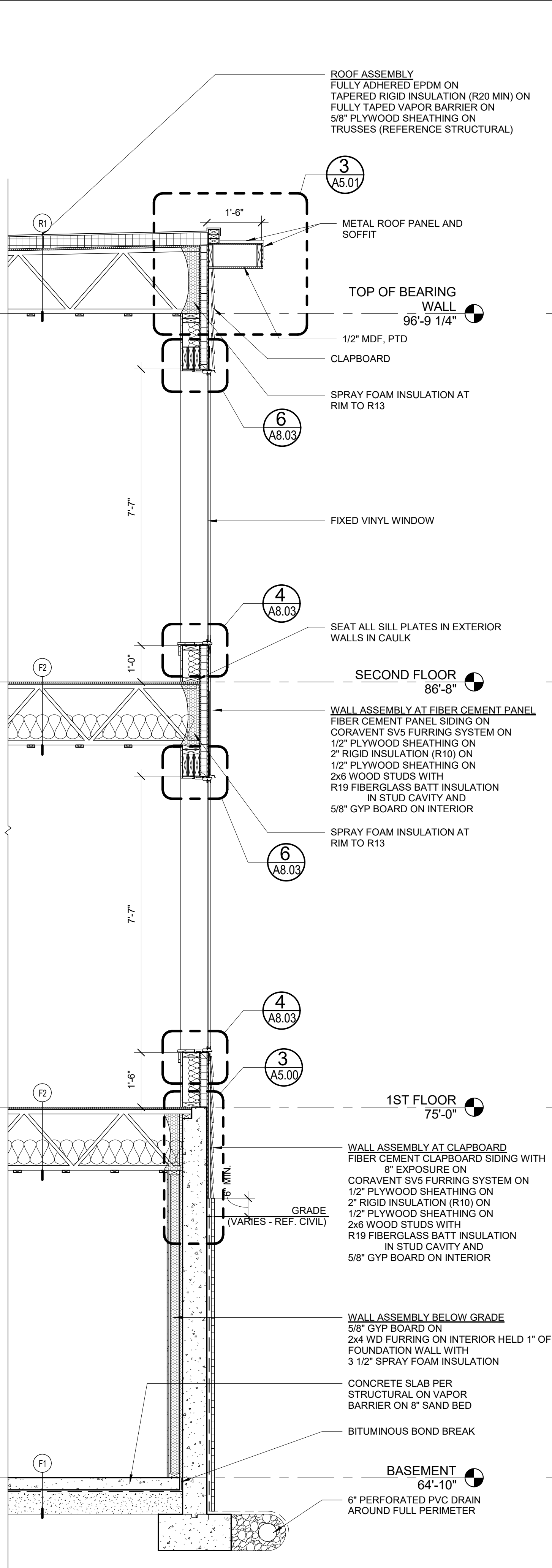
3 | WALL SECTION AT WEST END 1/2" = 1'-0"
