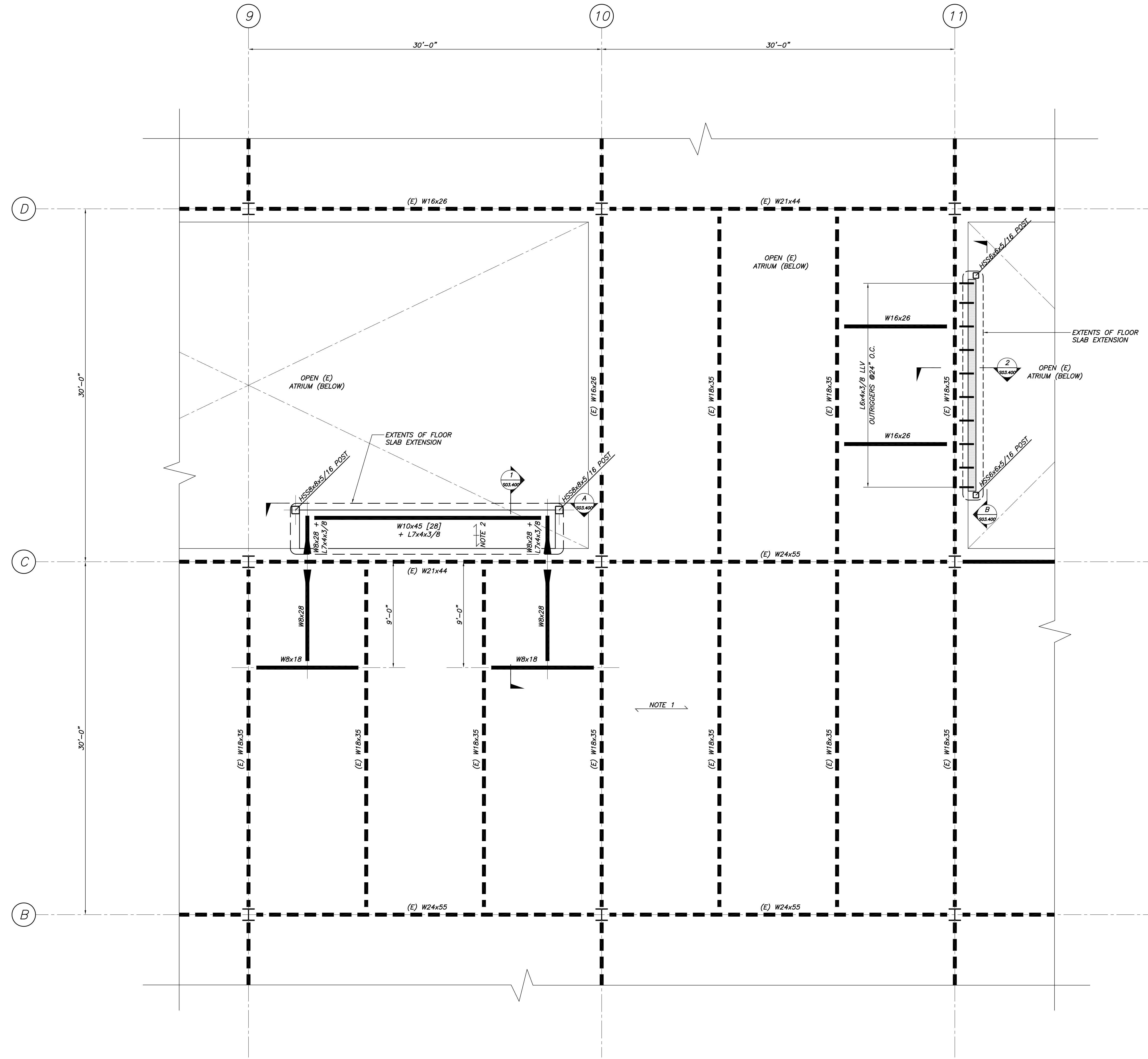
PARTIAL LEVEL 02 FRAMING PLAN 1/4"=1'-0"
