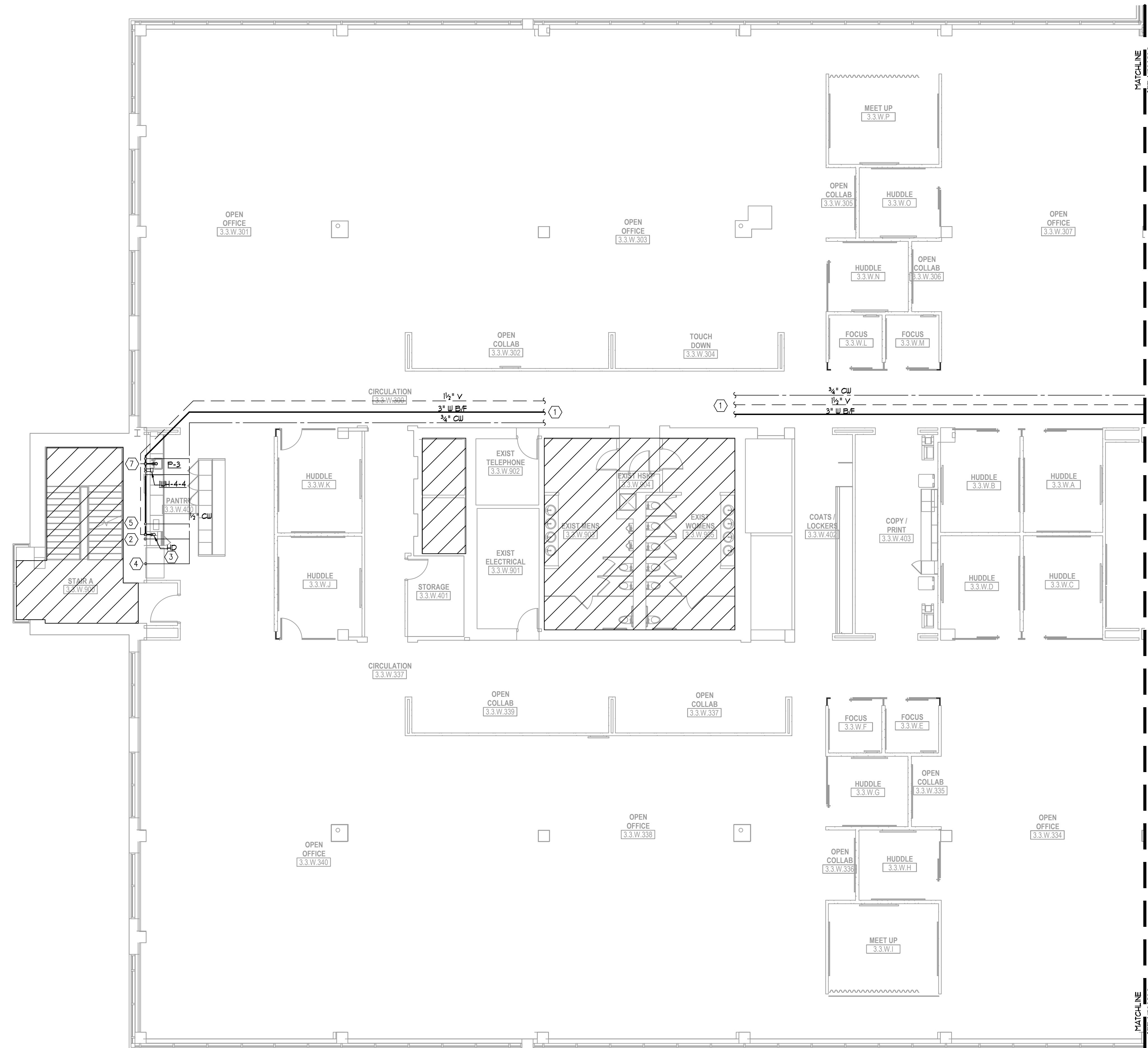
2 3RD FLOOR PLAN - PLUMBING P3.103W 1/8" = 1'-0"
