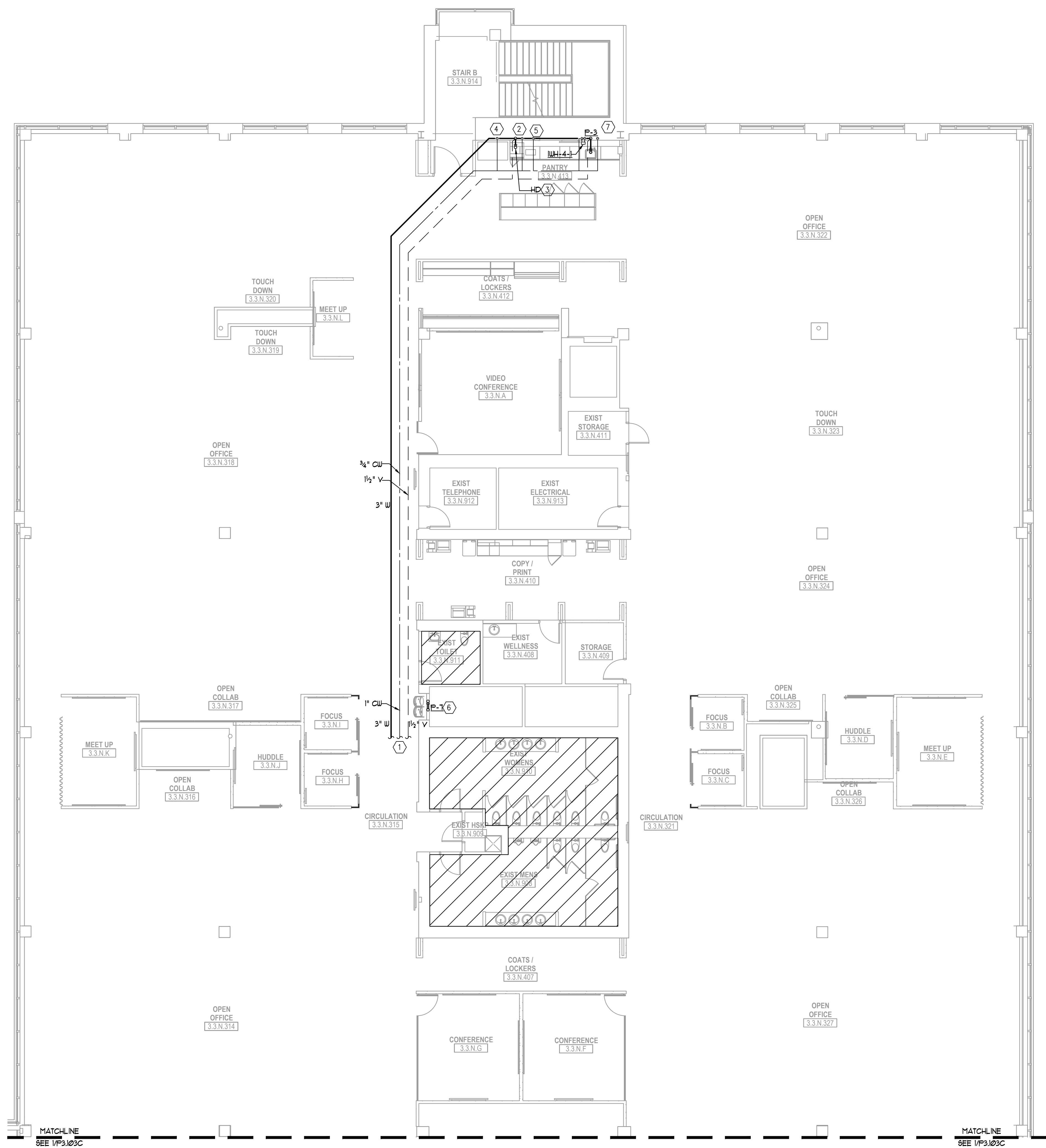
2 3RD FLOOR PLAN - PLUMBING P3.103N 1/8" = 1'-0"
