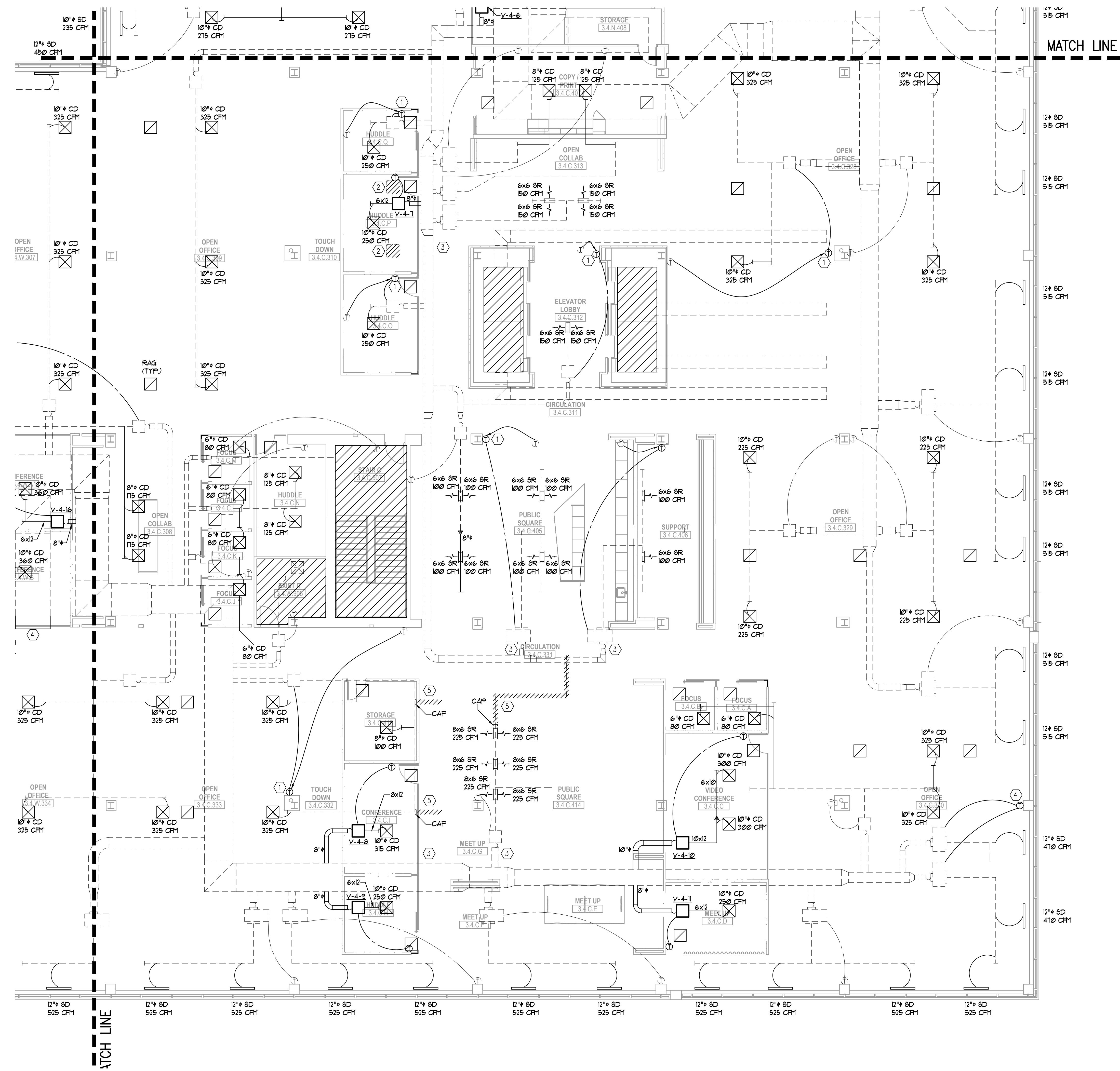
1 4TH FLOOR PLAN - HVAC 2.104C 1/8"=1'-0"
