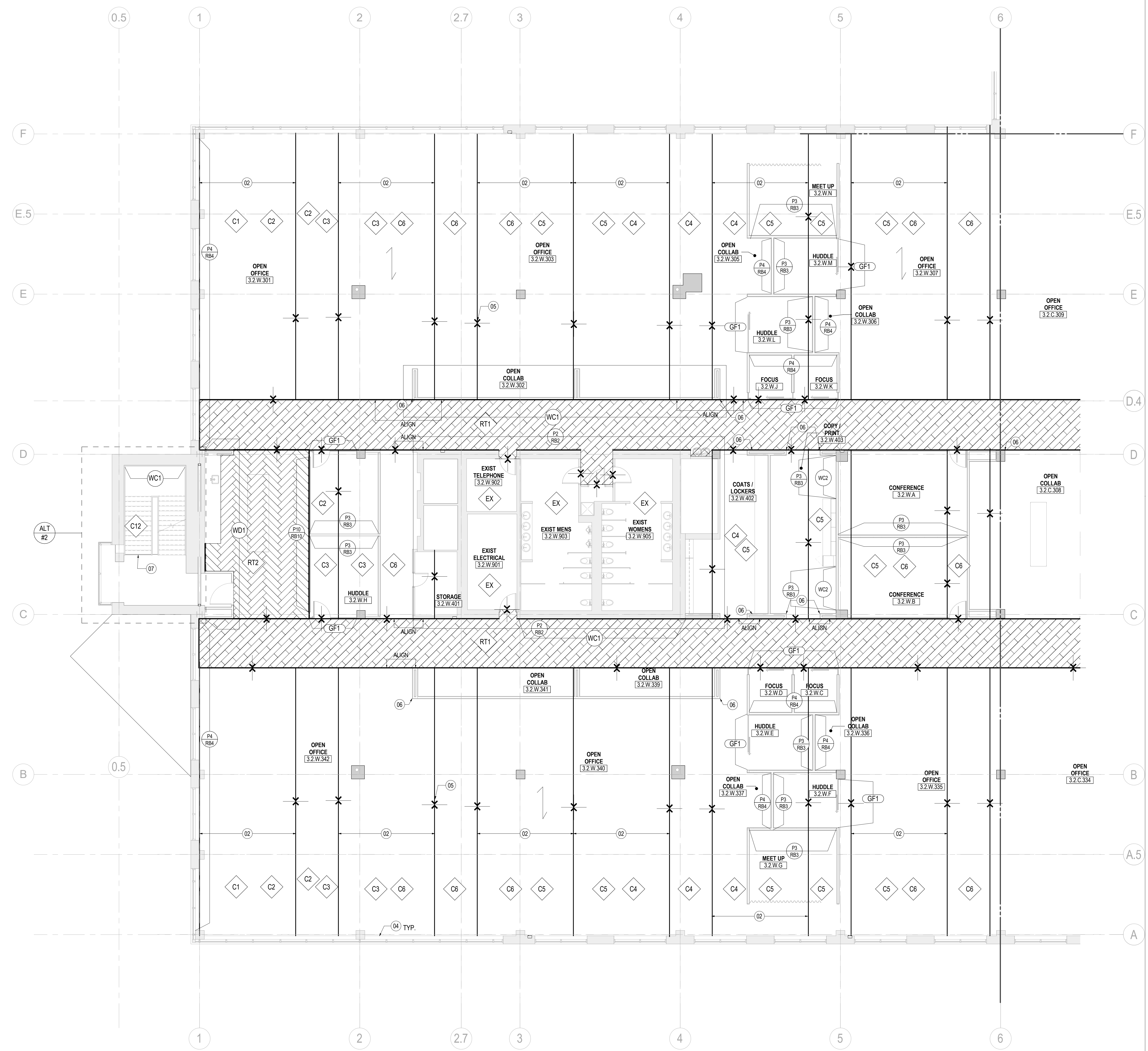
2 FINISH PLAN - LEVEL 02 - AREA W SCALE: 1/8" = 1'-0"
