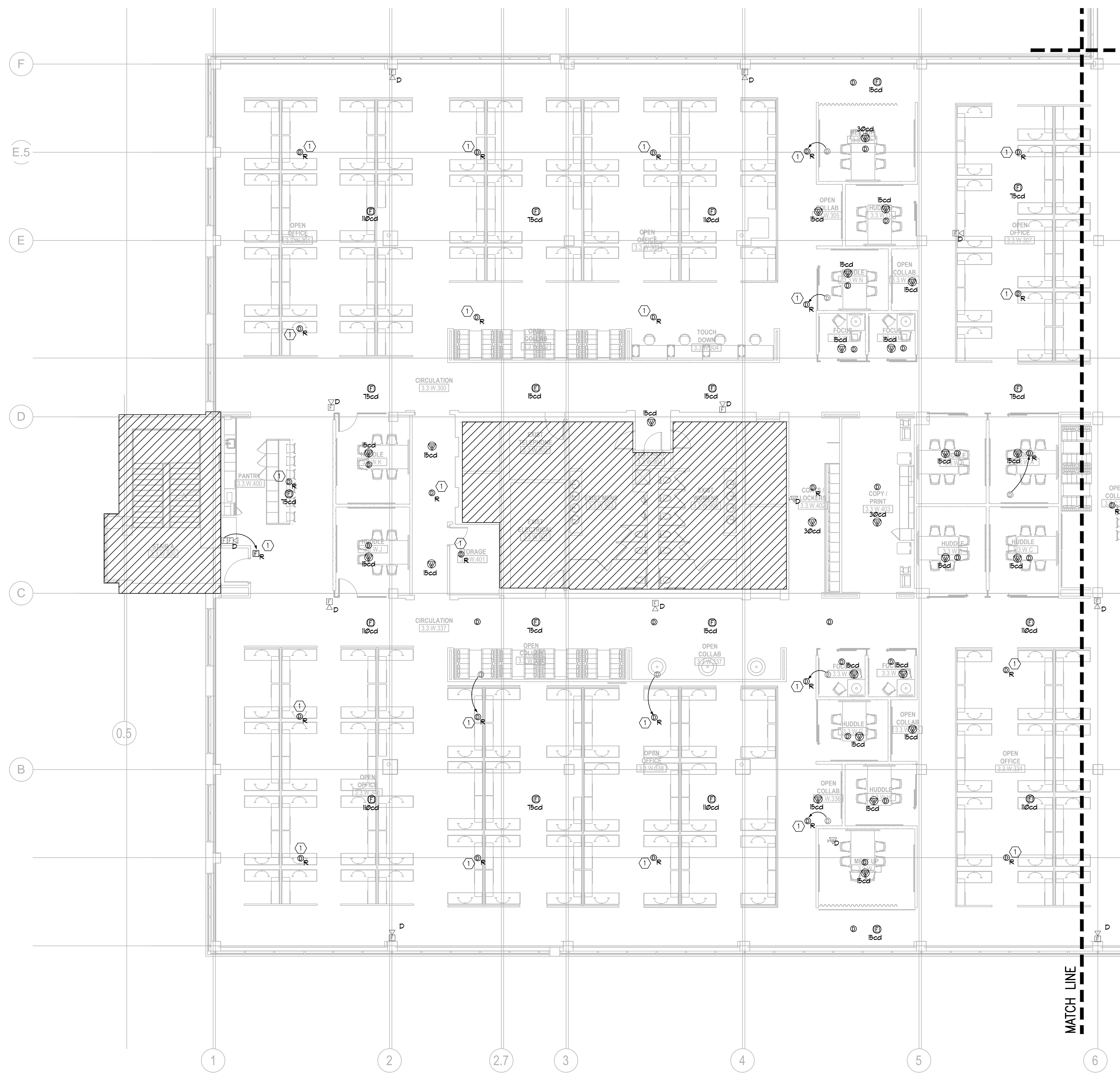
3RD FLOOR PLAN (AREA W) - FIRE ALARM E3.303W 1/8" = 1'-0"
