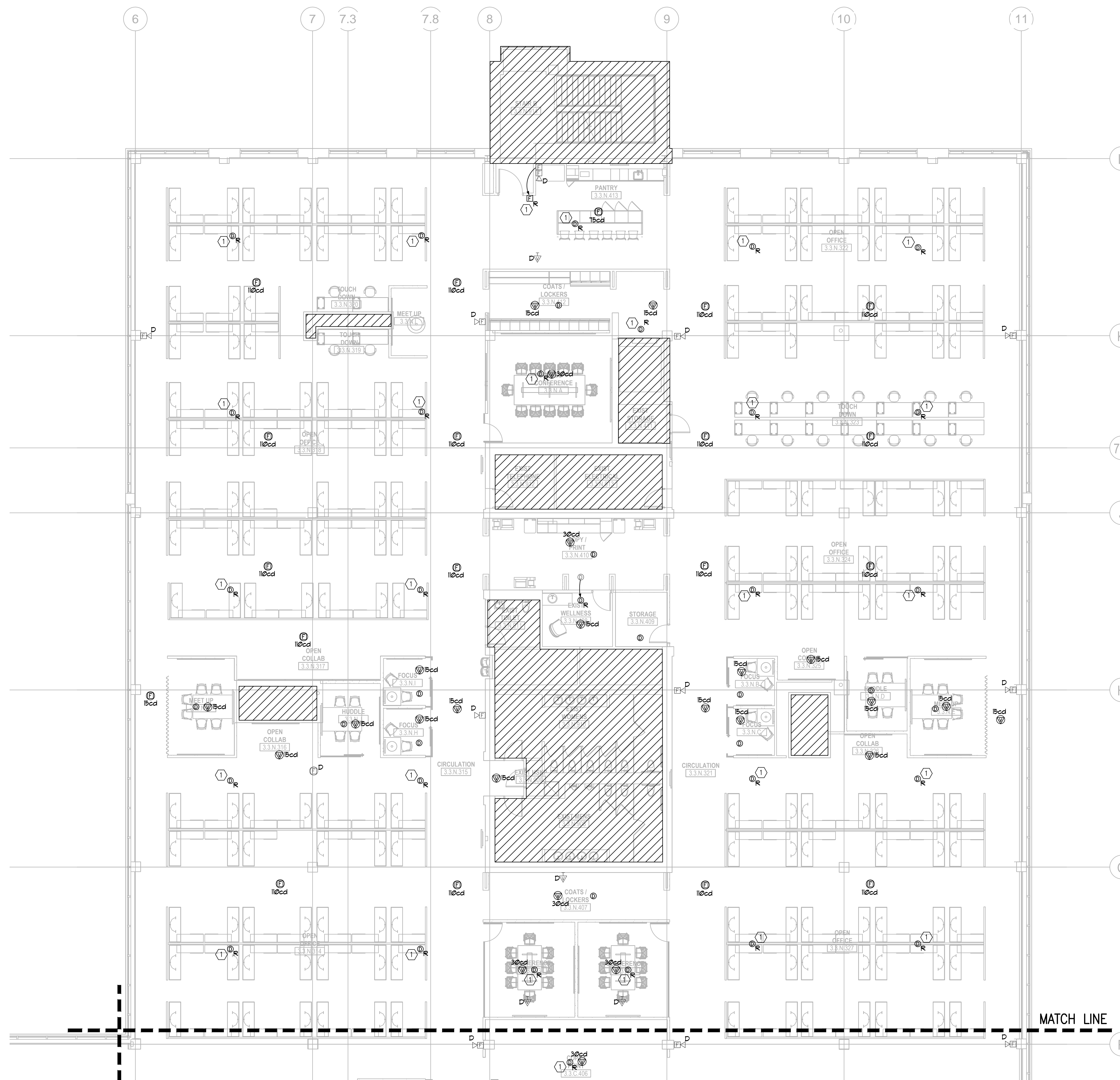
1 3RD FLOOR PLAN (AREA N) -- FIRE ALARM E3.303N 1/8"=1'-0"
