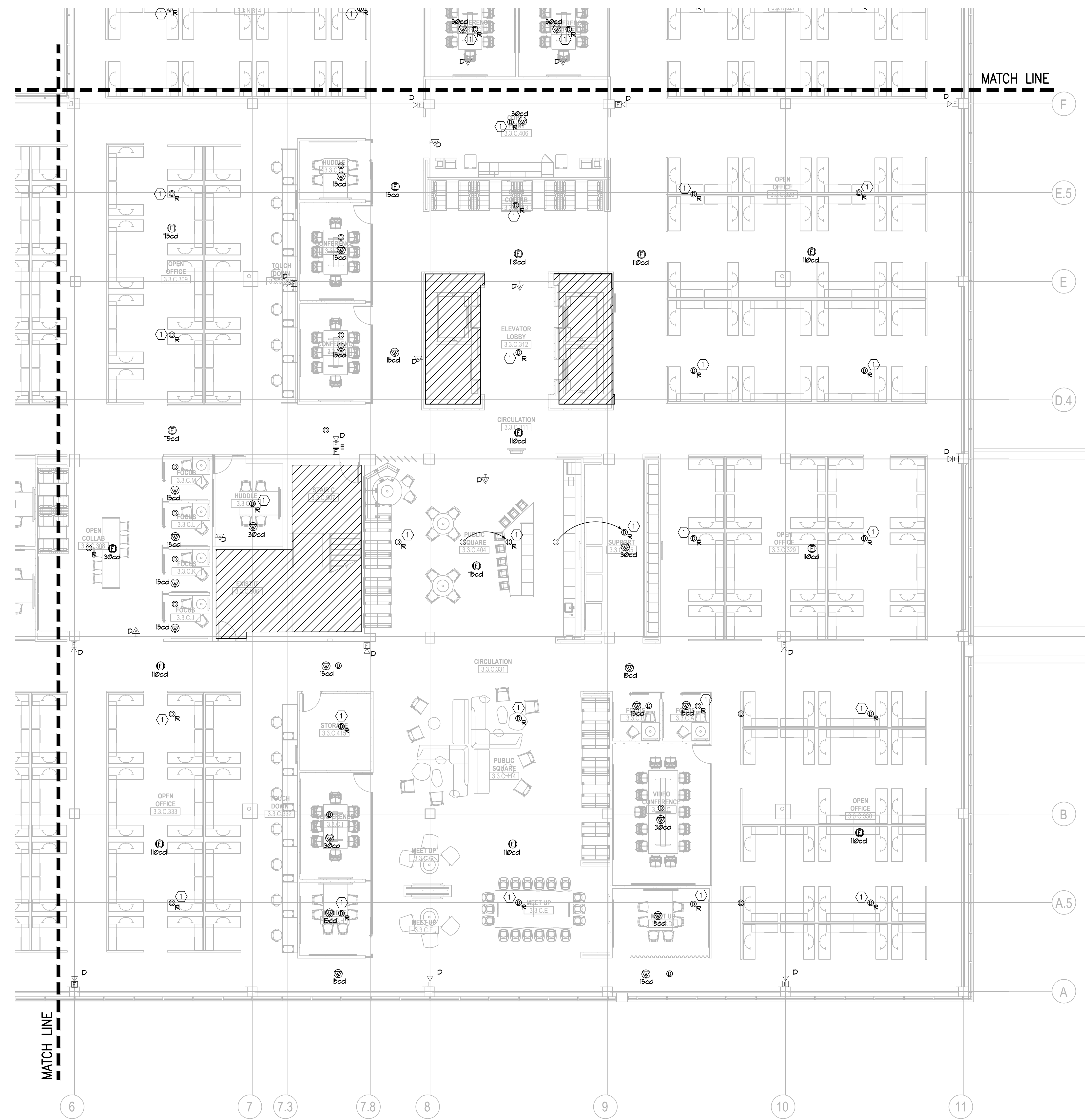
① 3RD FLOOR PLAN (AREA C) - FIRE ALARM E3.303C 1/8" = 1'-0"
