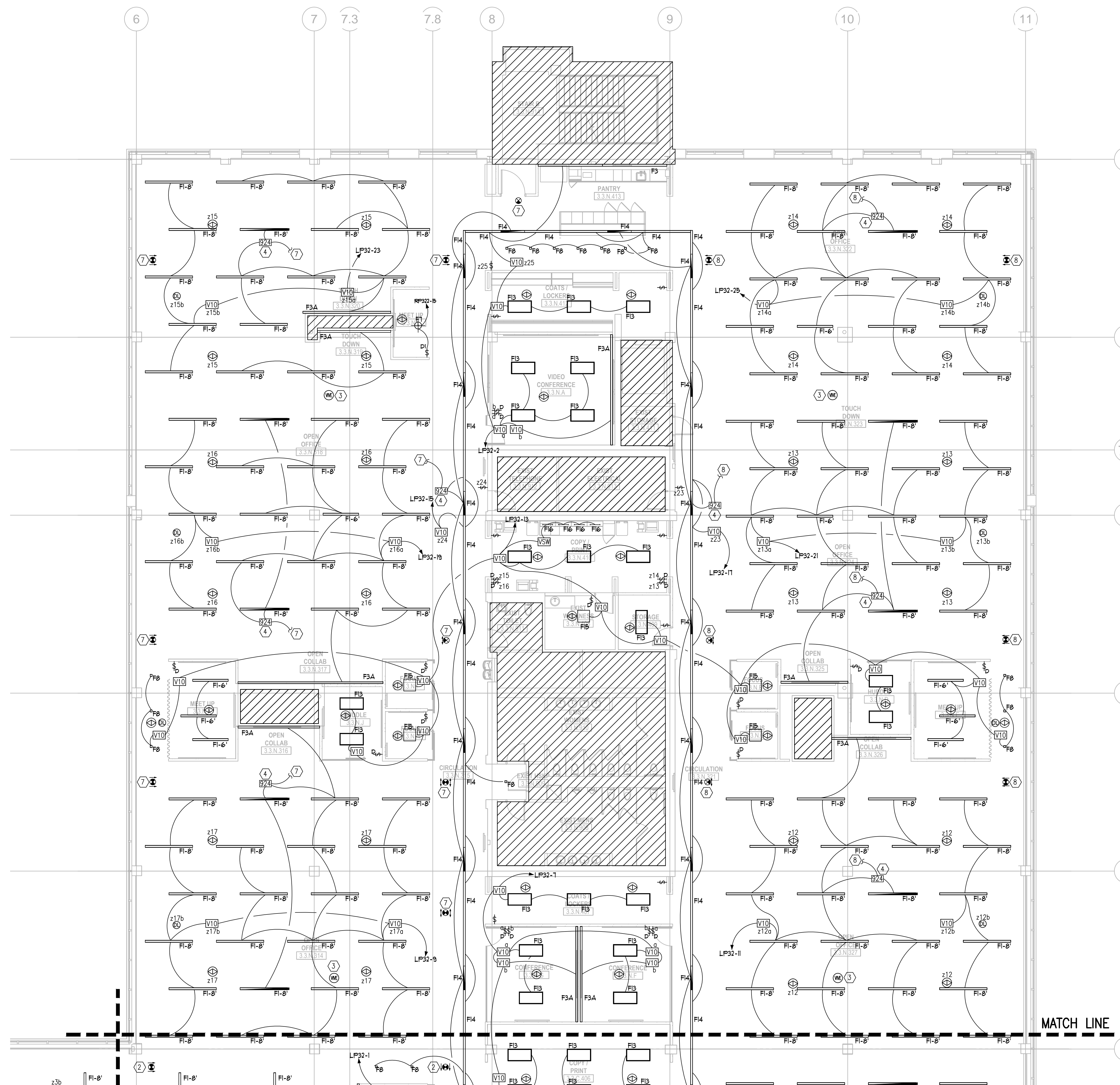
1 3RD FLOOR PLAN (AREA N) - LIGHTING E3.203N 1/8"=1'-0"
