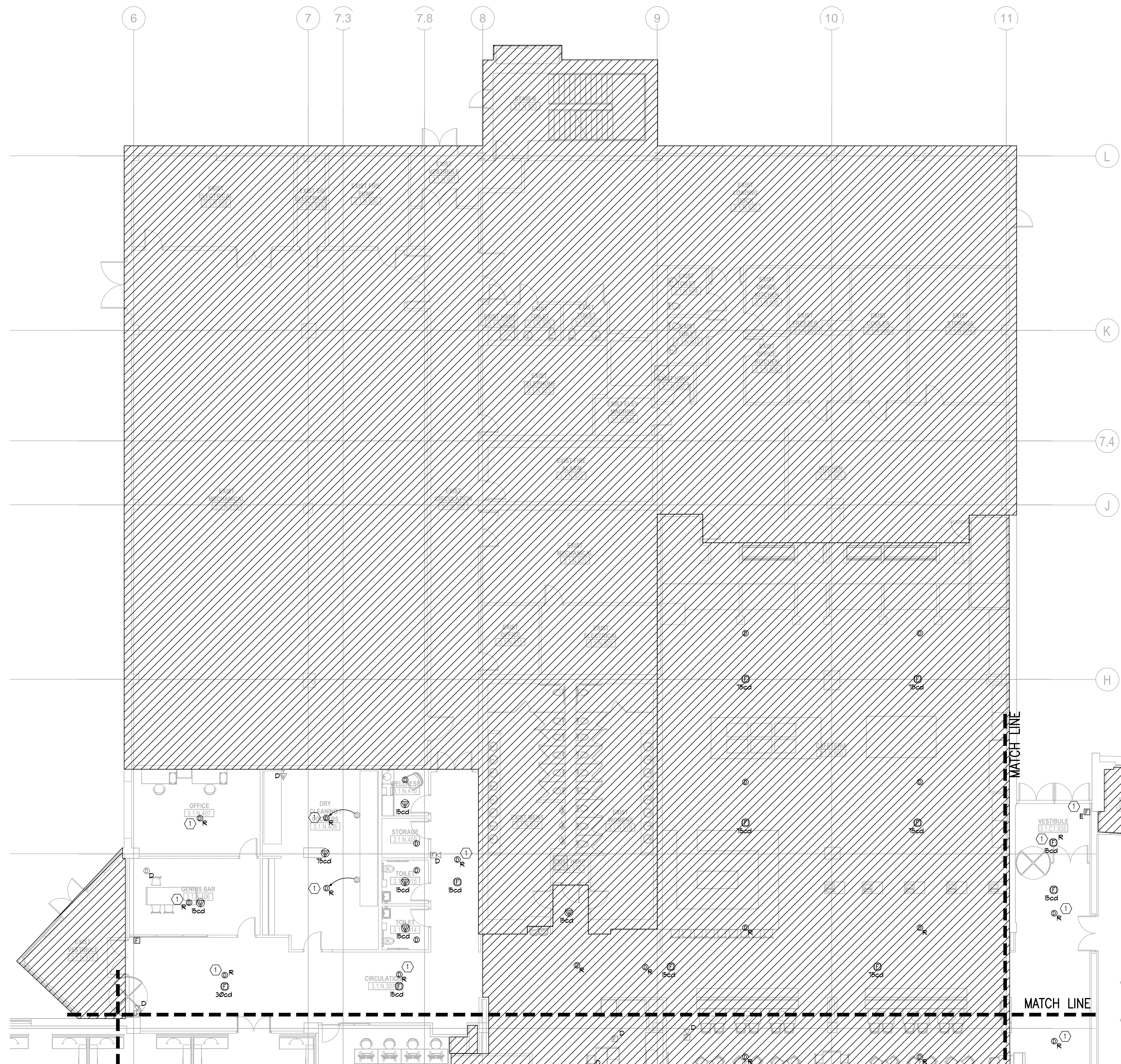
E2.301N 1ST FLOOR PLAN (AREA N) - FIRE ALARM 1/8" = 1'-0"
