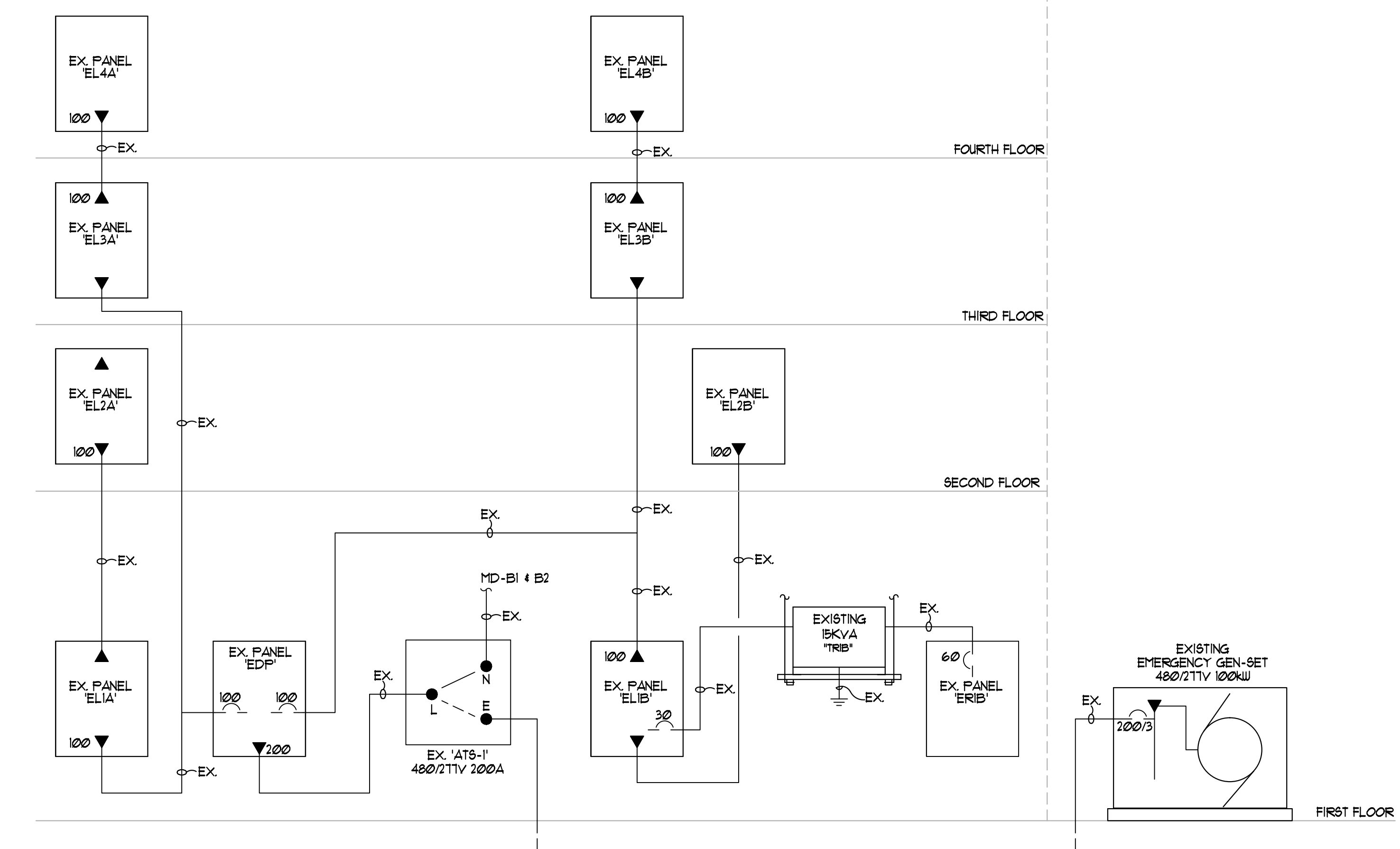
HO3 BUILDING EMERGENCY POWER RISER DIAGRAM PARTIAL E2.500 NOT TO SCALE
