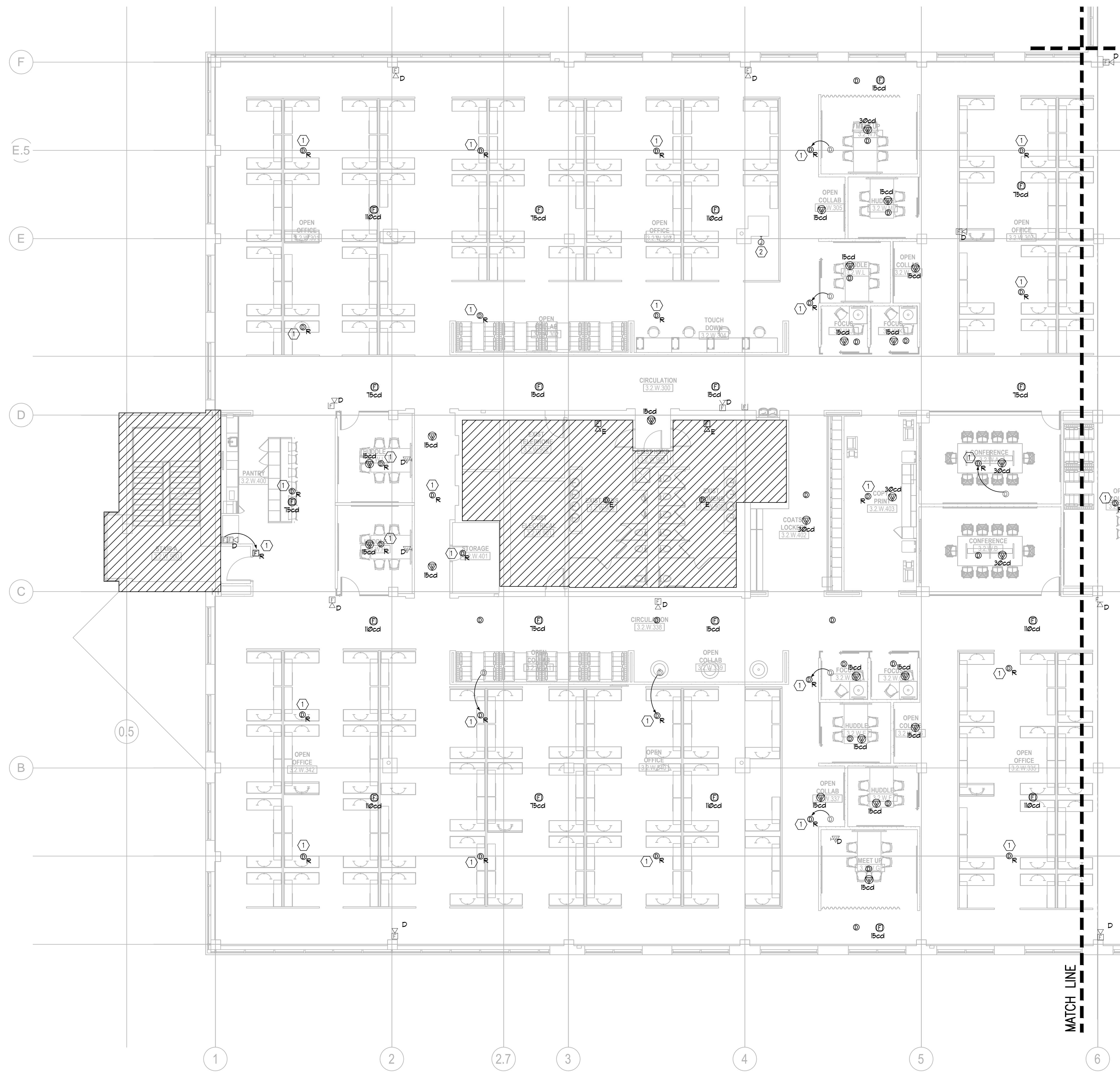
1 2ND FLOOR PLAN (AREA W) - FIRE ALARM E2.302W 1/8" = 1'-0"
